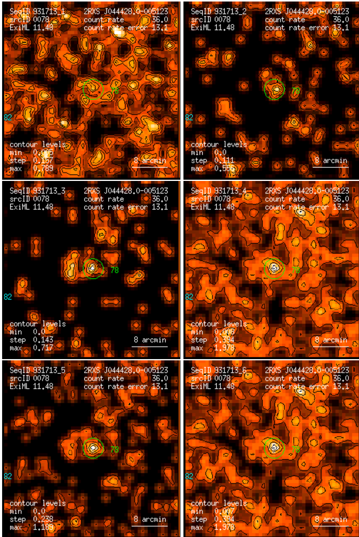
Figure 78: RASS 931713: detection 0078: band rate images, Gaussian filter: (1) PSPC channels 11 – 41, (2) 52 – 90, (3) 91 – 201, (4) 11 – 235, (5) 52 – 201, (6) 11 – 201. Broad band rates in counts/ks. Band rate contour levels in counts/ks/arcmin 2 .
