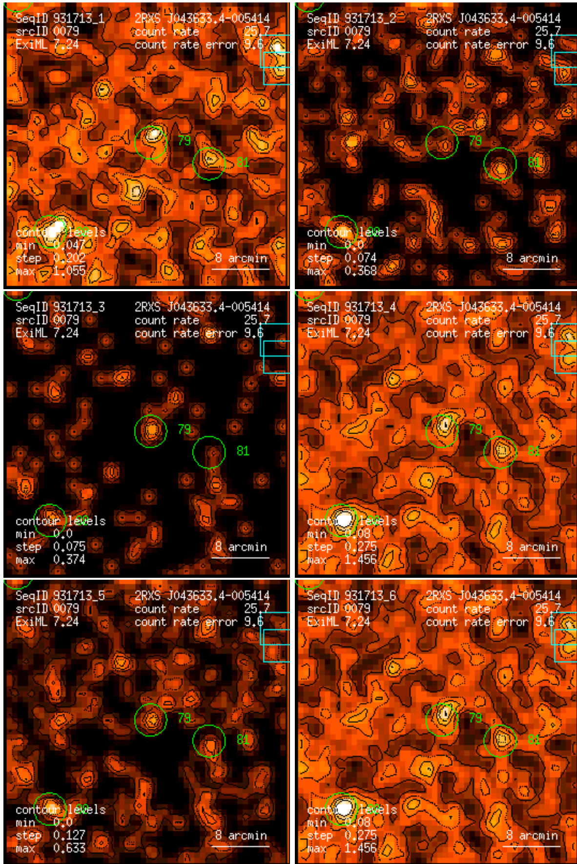
Figure 79: RASS 931713: detection 0079: band rate images, Gaussian filter: (1) PSPC channels 11 – 41, (2) 52 – 90, (3) 91 – 201, (4) 11 – 235, (5) 52 – 201, (6) 11 – 201. Broad band rates in counts/ks. Band rate contour levels in counts/ks/arcmin 2 .
