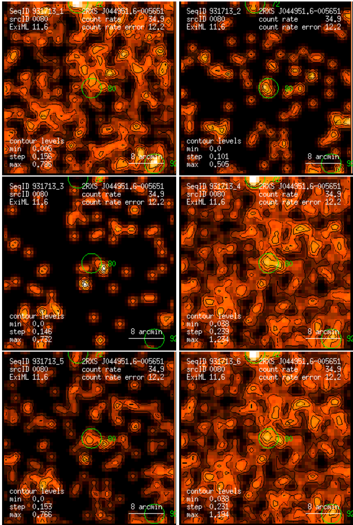
Figure 80: RASS 931713: detection 0080: band rate images, Gaussian filter: (1) PSPC channels 11 – 41, (2) 52 – 90, (3) 91 – 201, (4) 11 – 235, (5) 52 – 201, (6) 11 – 201. Broad band rates in counts/ks. Band rate contour levels in counts/ks/arcmin 2 .
