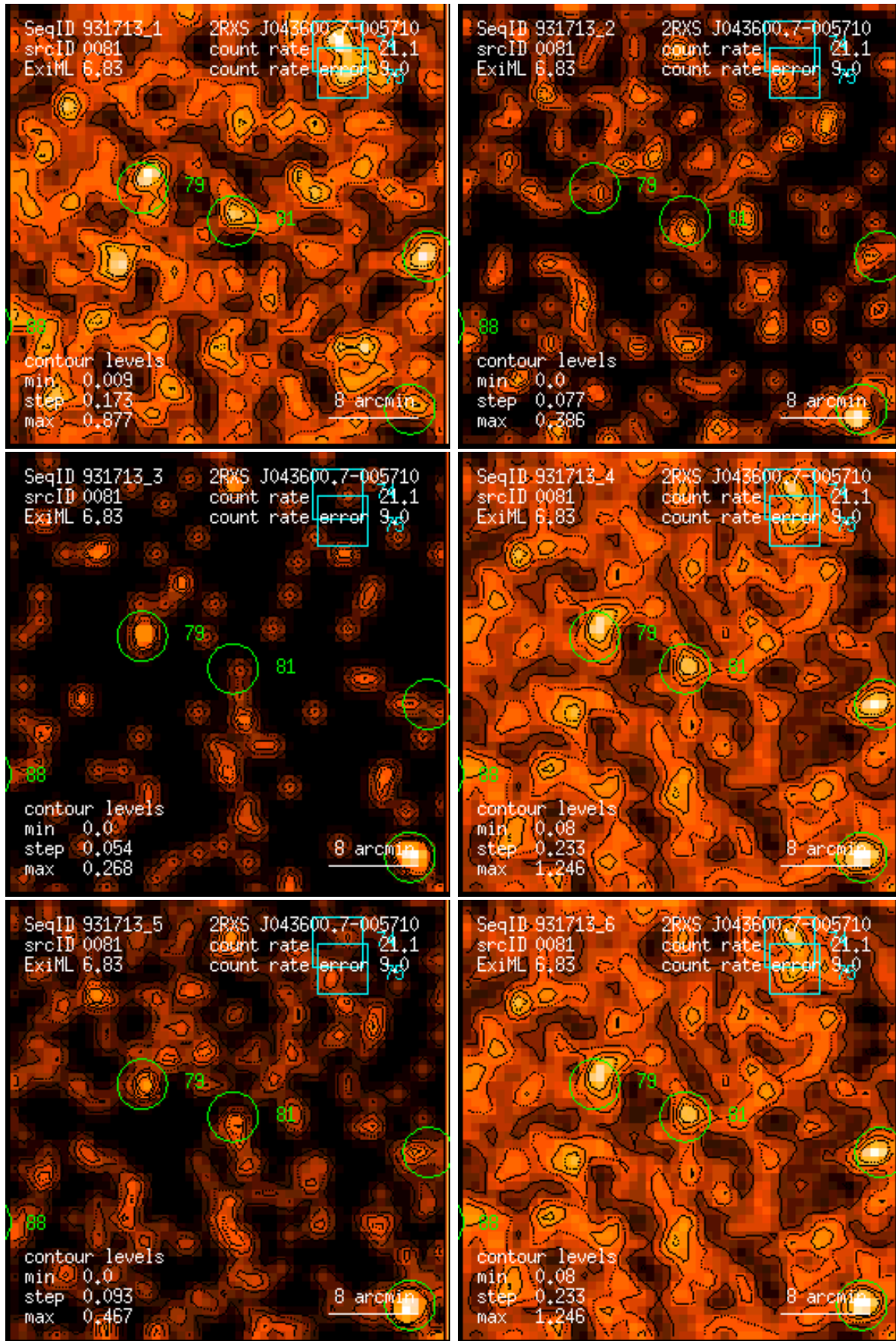
Figure 81: RASS 931713: detection 0081: band rate images, Gaussian filter: (1) PSPC channels 11 – 41, (2) 52 – 90, (3) 91 – 201, (4) 11 – 235, (5) 52 – 201, (6) 11 – 201. Broad band rates in counts/ks. Band rate contour levels in counts/ks/arcmin 2 .
