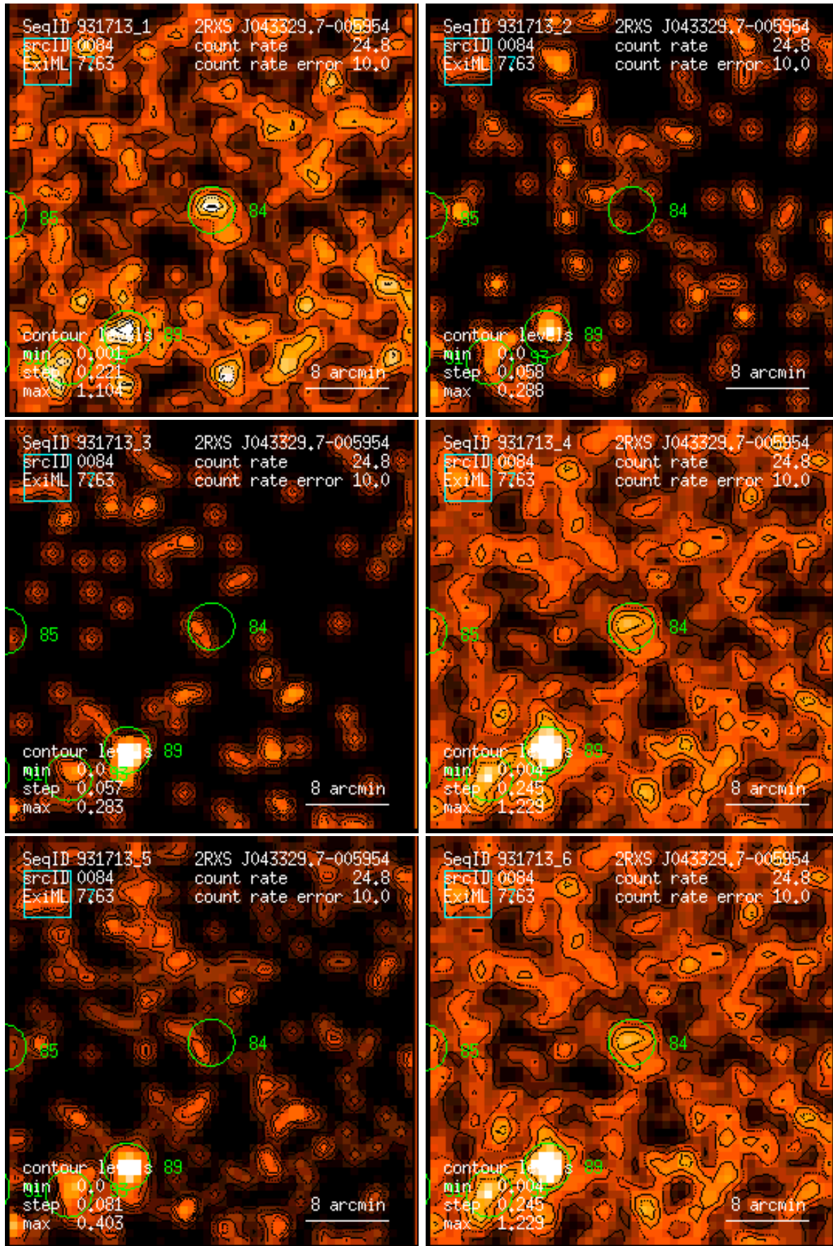
Figure 84: RASS 931713: detection 0084: band rate images, Gaussian filter: (1) PSPC channels 11 – 41, (2) 52 – 90, (3) 91 – 201, (4) 11 – 235, (5) 52 – 201, (6) 11 – 201. Broad band rates in counts/ks. Band rate contour levels in counts/ks/arcmin 2 .
