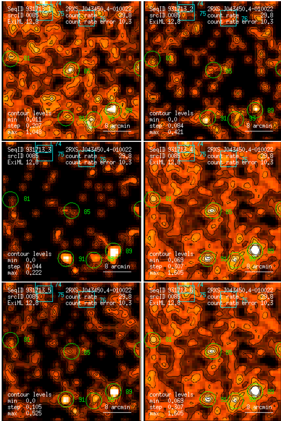
Figure 85: RASS 931713: detection 0085: band rate images, Gaussian filter: (1) PSPC channels 11 – 41, (2) 52 – 90, (3) 91 – 201, (4) 11 – 235, (5) 52 – 201, (6) 11 – 201. Broad band rates in counts/ks. Band rate contour levels in counts/ks/arcmin 2 .
