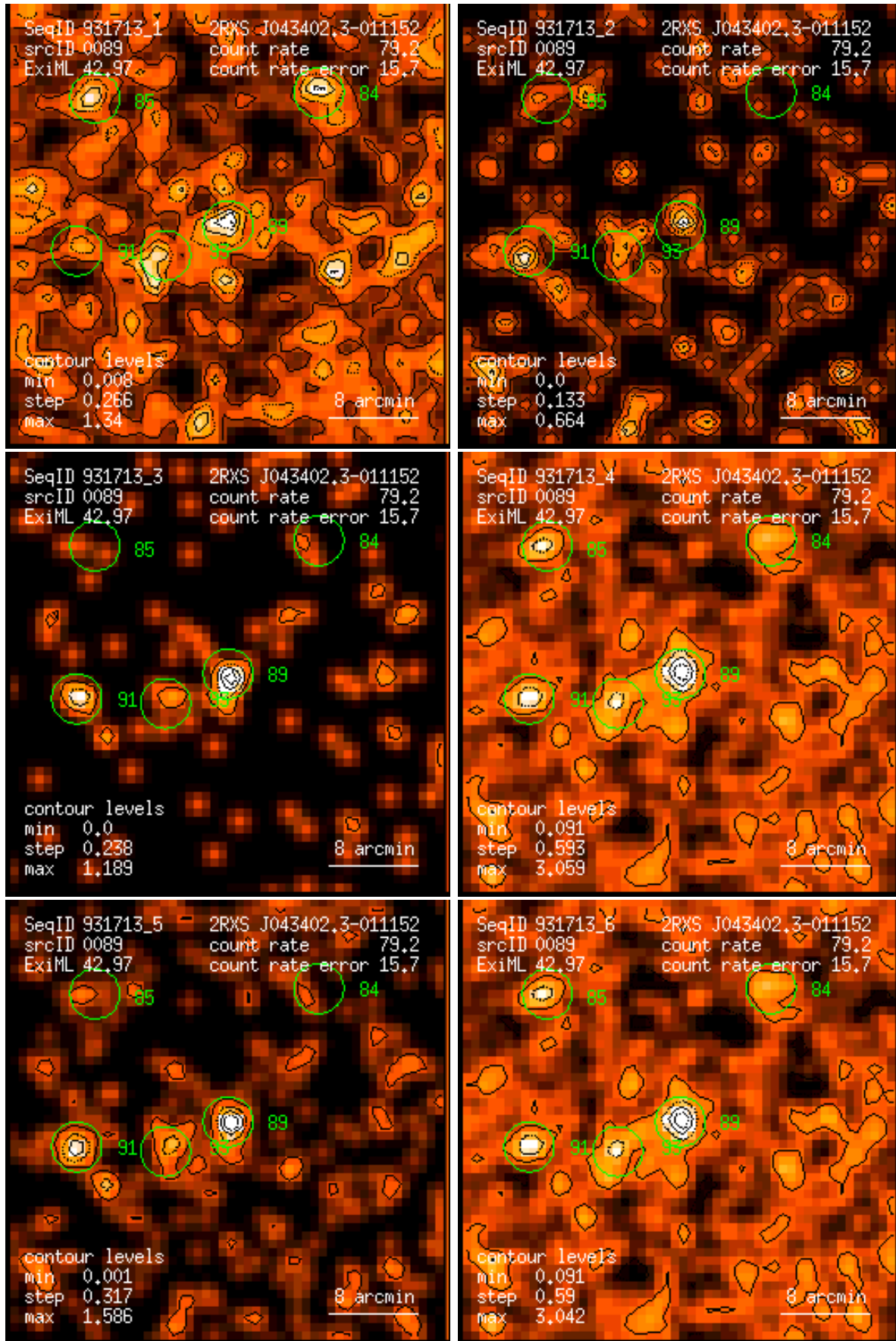
Figure 89: RASS 931713: detection 0089: band rate images, Gaussian filter: (1) PSPC channels 11 – 41, (2) 52 – 90, (3) 91 – 201, (4) 11 – 235, (5) 52 – 201, (6) 11 – 201. Broad band rates in counts/ks. Band rate contour levels in counts/ks/arcmin 2 .
