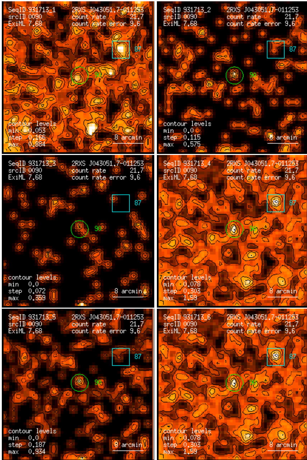
Figure 90: RASS 931713: detection 0090: band rate images, Gaussian filter: (1) PSPC channels 11 – 41, (2) 52 – 90, (3) 91 – 201, (4) 11 – 235, (5) 52 – 201, (6) 11 – 201. Broad band rates in counts/ks. Band rate contour levels in counts/ks/arcmin 2 .
