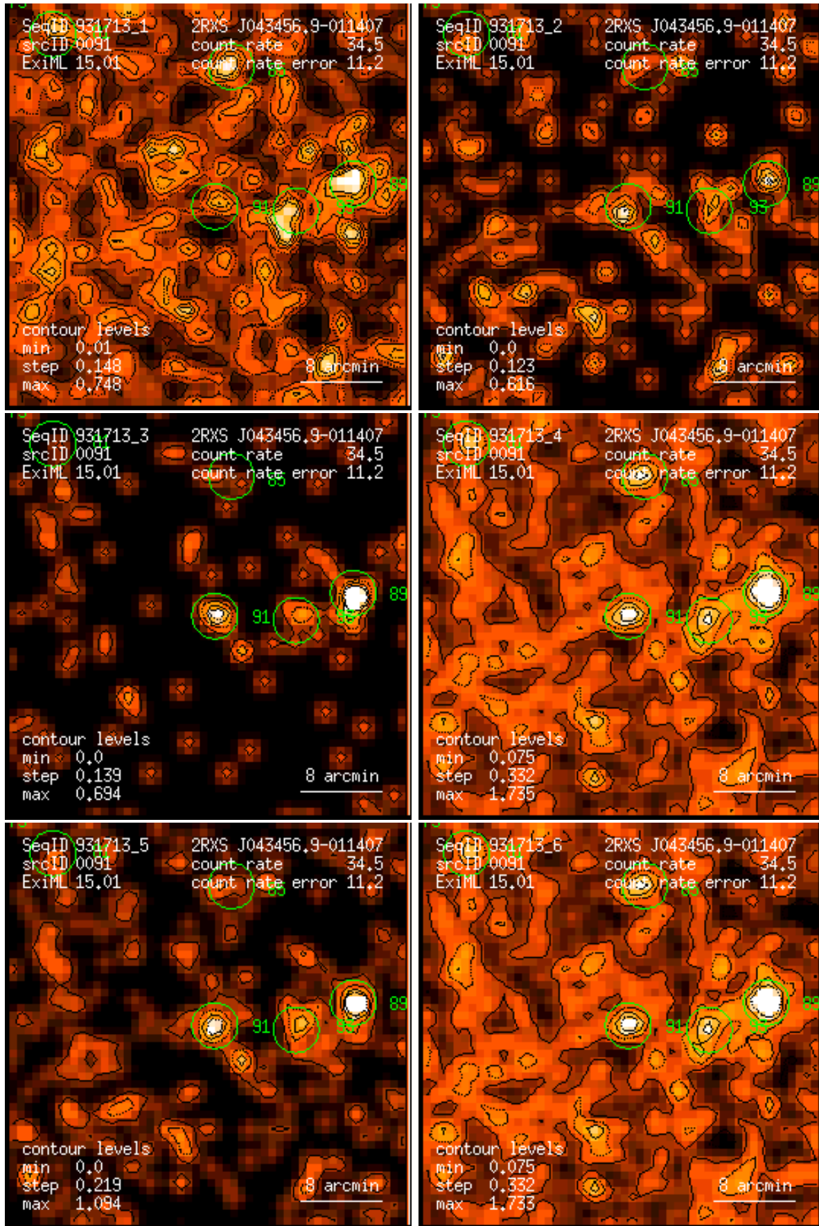
Figure 91: RASS 931713: detection 0091: band rate images, Gaussian filter: (1) PSPC channels 11 – 41, (2) 52 – 90, (3) 91 – 201, (4) 11 – 235, (5) 52 – 201, (6) 11 – 201. Broad band rates in counts/ks. Band rate contour levels in counts/ks/arcmin 2 .
