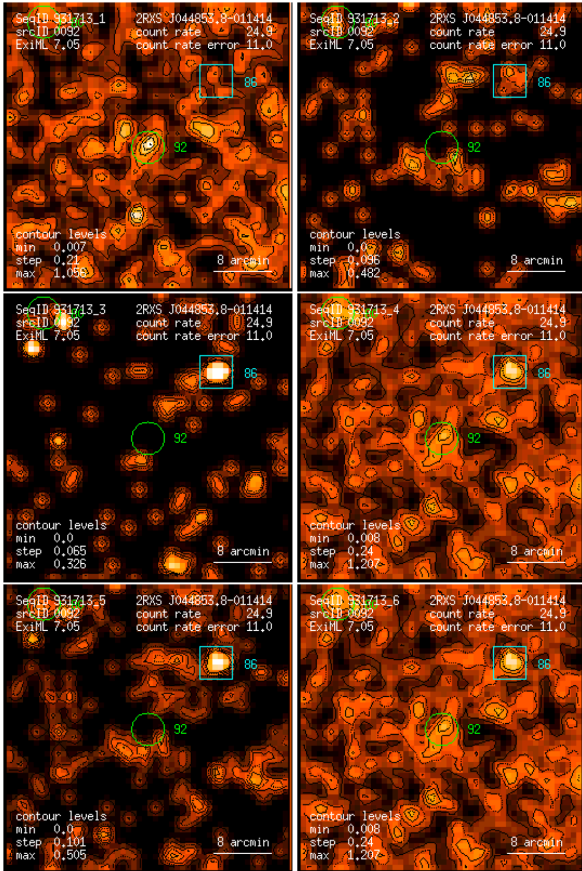
Figure 92: RASS 931713: detection 0092: band rate images, Gaussian filter: (1) PSPC channels 11 – 41, (2) 52 – 90, (3) 91 – 201, (4) 11 – 235, (5) 52 – 201, (6) 11 – 201. Broad band rates in counts/ks. Band rate contour levels in counts/ks/arcmin 2 .
