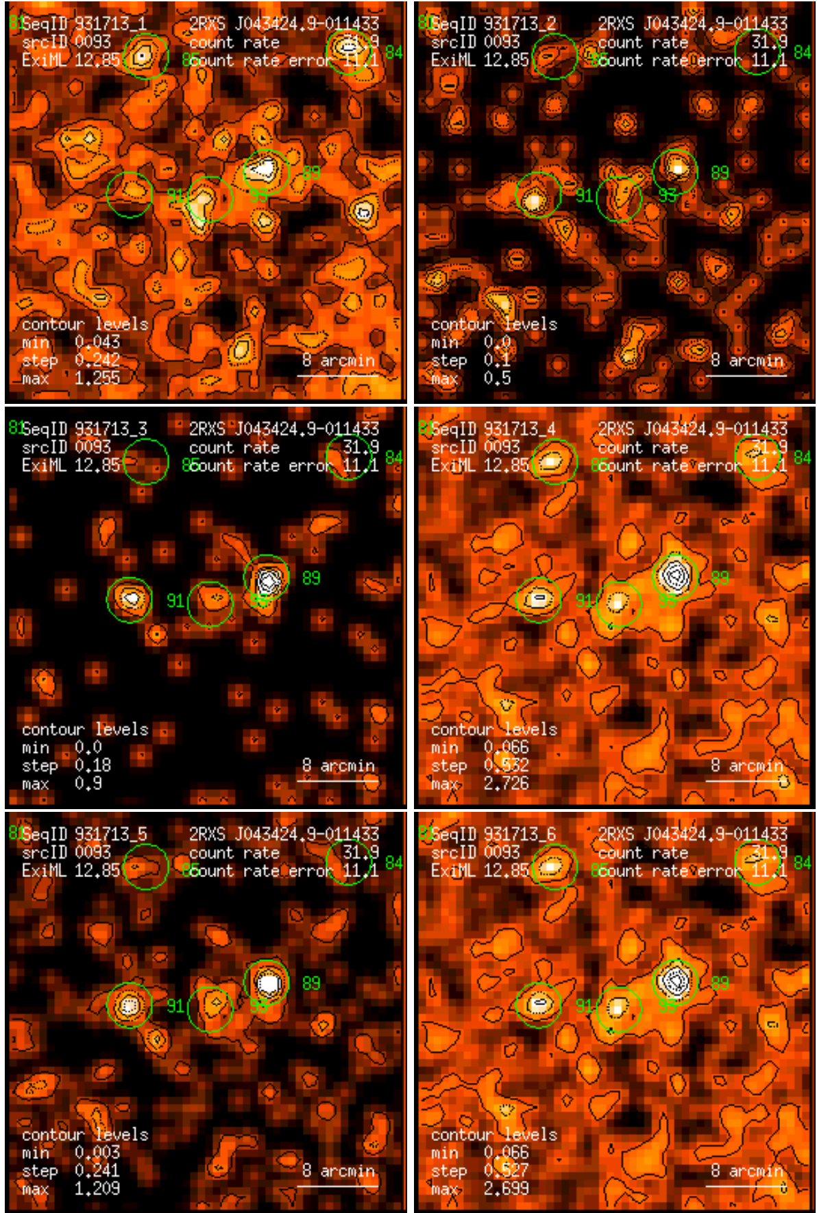
Figure 93: RASS 931713: detection 0093: band rate images, Gaussian filter: (1) PSPC channels 11 – 41, (2) 52 – 90, (3) 91 – 201, (4) 11 – 235, (5) 52 – 201, (6) 11 – 201. Broad band rates in counts/ks. Band rate contour levels in counts/ks/arcmin 2 .
