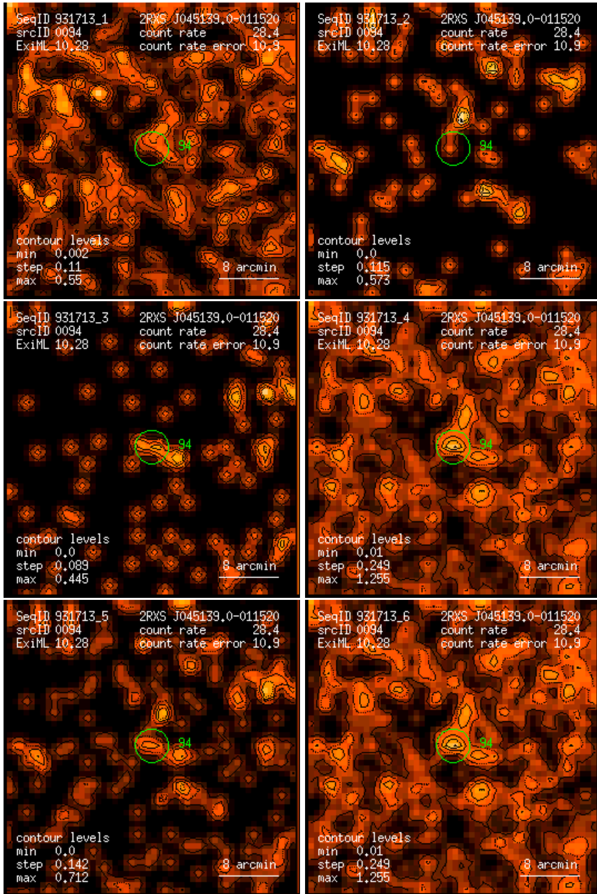
Figure 94: RASS 931713: detection 0094: band rate images, Gaussian filter: (1) PSPC channels 11 – 41, (2) 52 – 90, (3) 91 – 201, (4) 11 – 235, (5) 52 – 201, (6) 11 – 201. Broad band rates in counts/ks. Band rate contour levels in counts/ks/arcmin 2 .
