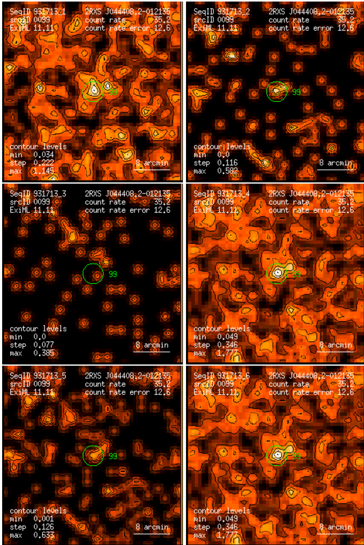
Figure 99: RASS 931713: detection 0099: band rate images, Gaussian filter: (1) PSPC channels 11 – 41, (2) 52 – 90, (3) 91 – 201, (4) 11 – 235, (5) 52 – 201, (6) 11 – 201. Broad band rates in counts/ks. Band rate contour levels in counts/ks/arcmin 2 .
