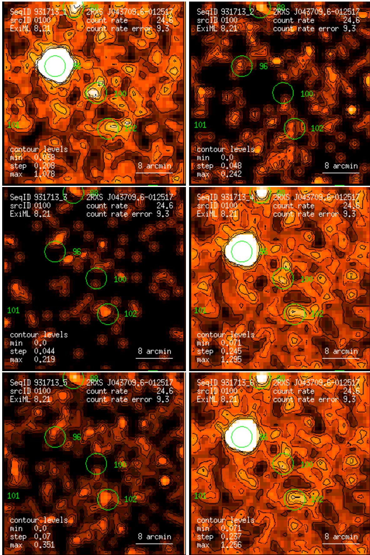
Figure 100: RASS 931713: detection 0100: band rate images, Gaussian filter: (1) PSPC channels 11 – 41, (2) 52 – 90, (3) 91 – 201, (4) 11 – 235, (5) 52 – 201, (6) 11 – 201. Broad band rates in counts/ks. Band rate contour levels in counts/ks/arcmin 2 .
