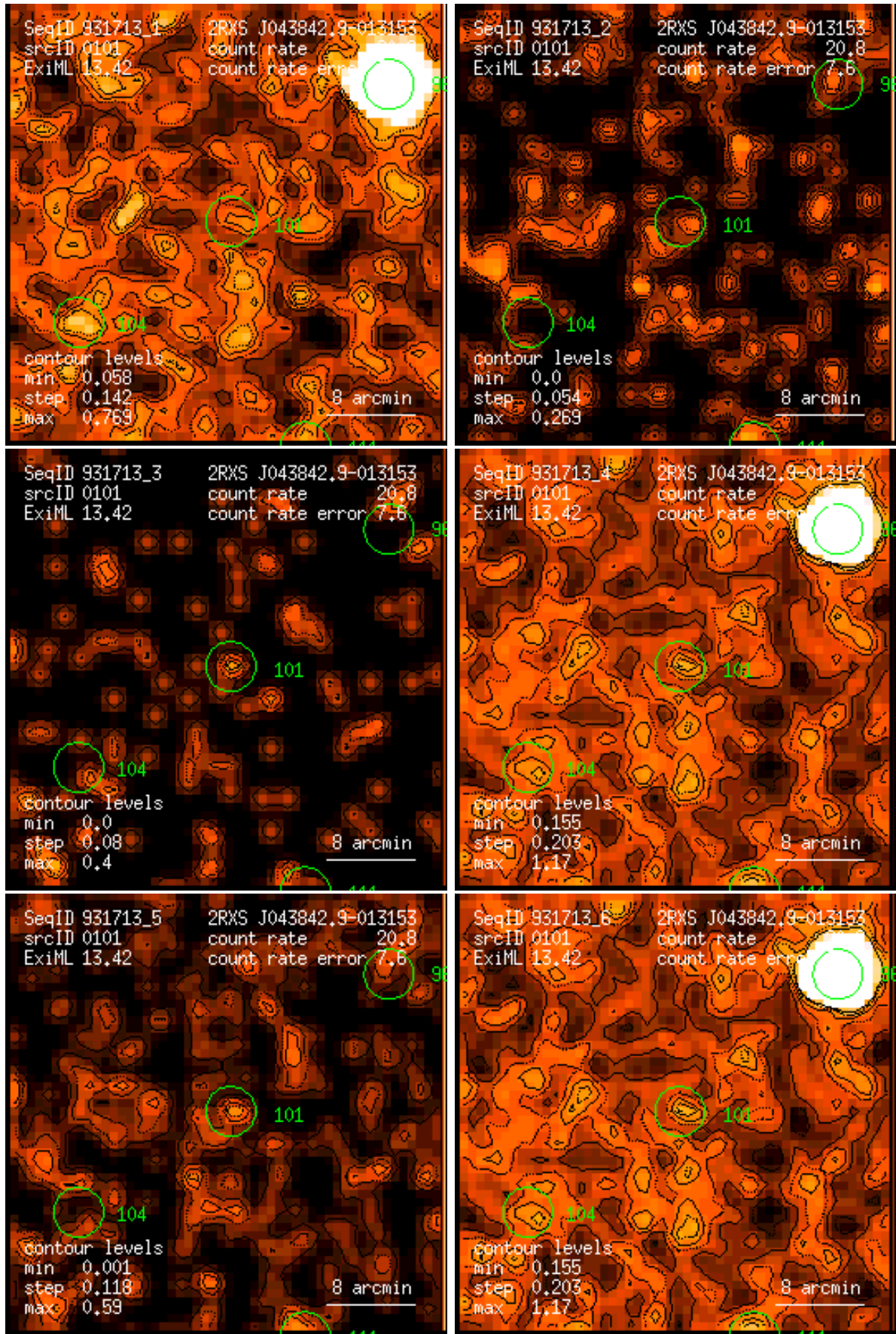
Figure 101: RASS 931713: detection 0101: band rate images, Gaussian filter: (1) PSPC channels 11 – 41, (2) 52 – 90, (3) 91 – 201, (4) 11 – 235, (5) 52 – 201, (6) 11 – 201. Broad band rates in counts/ks. Band rate contour levels in counts/ks/arcmin 2 .
