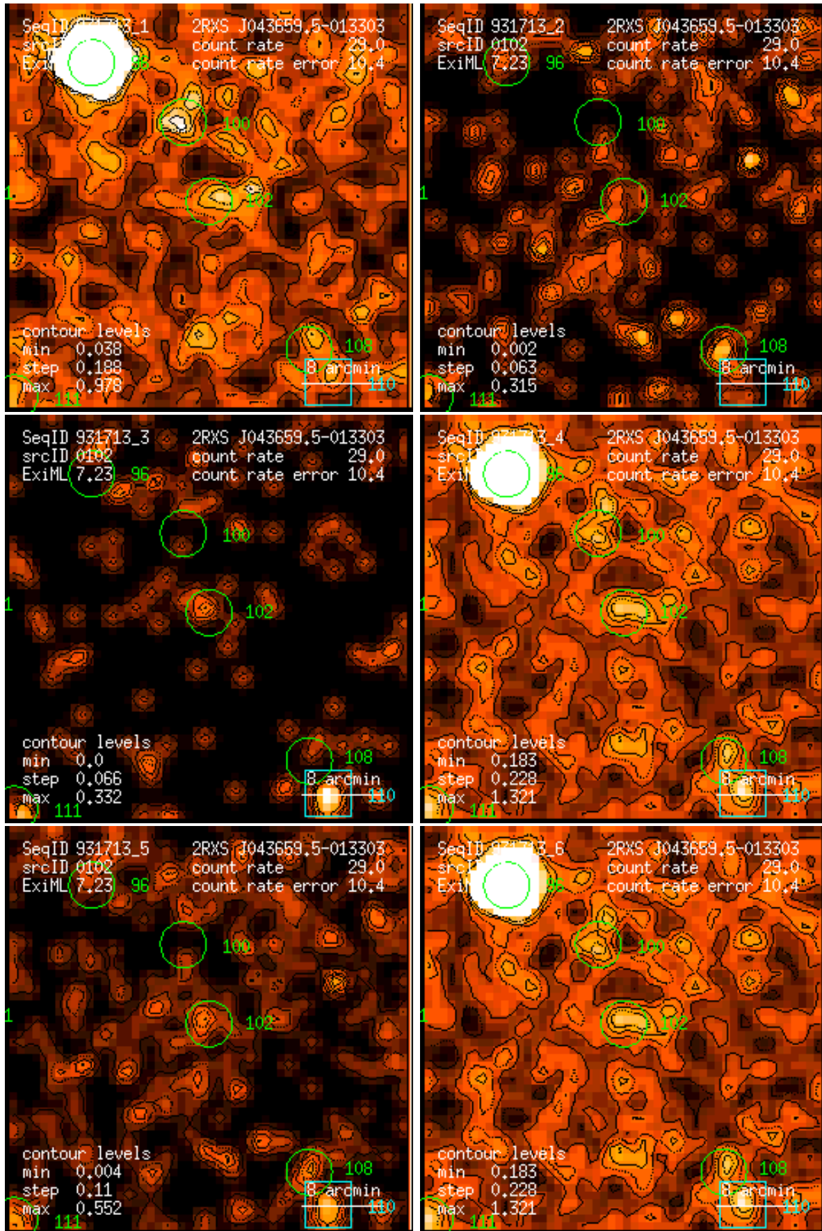
Figure 102: RASS 931713: detection 0102: band rate images, Gaussian filter: (1) PSPC channels 11 – 41, (2) 52 – 90, (3) 91 – 201, (4) 11 – 235, (5) 52 – 201, (6) 11 – 201. Broad band rates in counts/ks. Band rate contour levels in counts/ks/arcmin 2 .
