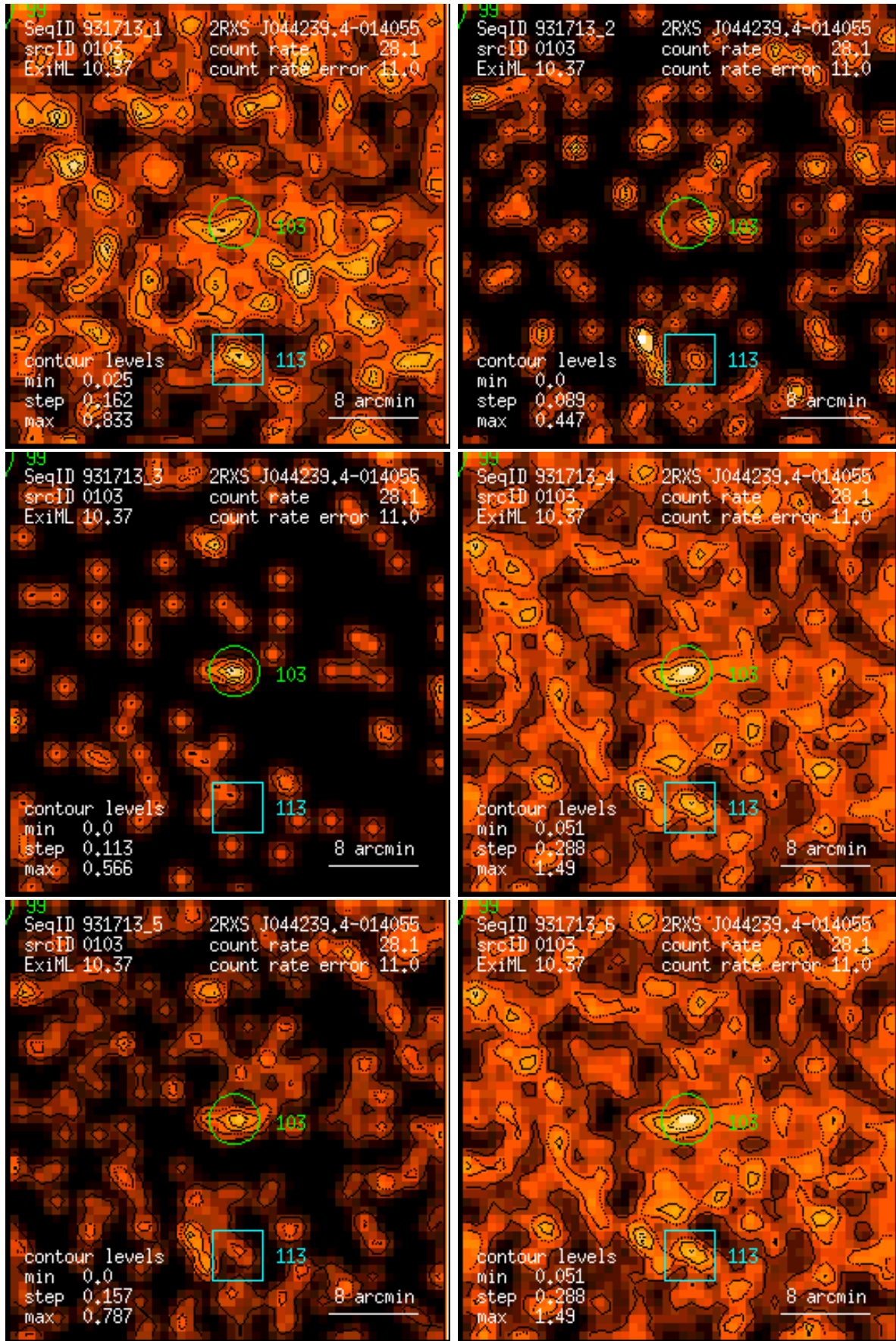
Figure 103: RASS 931713: detection 0103: band rate images, Gaussian filter: (1) PSPC channels 11 – 41, (2) 52 – 90, (3) 91 – 201, (4) 11 – 235, (5) 52 – 201, (6) 11 – 201. Broad band rates in counts/ks. Band rate contour levels in counts/ks/arcmin 2 .
