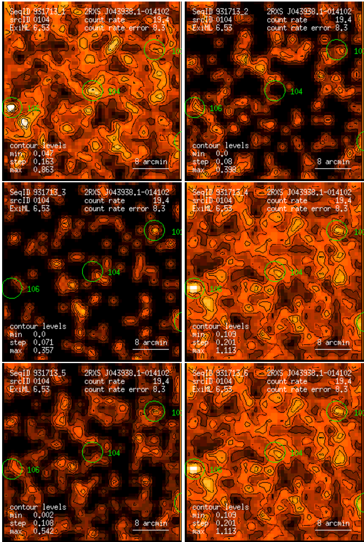
Figure 104: RASS 931713: detection 0104: band rate images, Gaussian filter: (1) PSPC channels 11 – 41, (2) 52 – 90, (3) 91 – 201, (4) 11 – 235, (5) 52 – 201, (6) 11 – 201. Broad band rates in counts/ks. Band rate contour levels in counts/ks/arcmin 2 .
