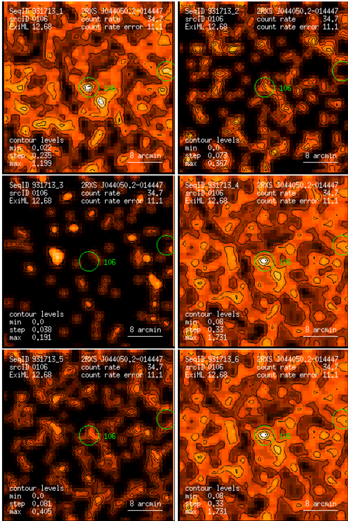
Figure 106: RASS 931713: detection 0106: band rate images, Gaussian filter: (1) PSPC channels 11 – 41, (2) 52 – 90, (3) 91 – 201, (4) 11 – 235, (5) 52 – 201, (6) 11 – 201. Broad band rates in counts/ks. Band rate contour levels in counts/ks/arcmin 2 .
