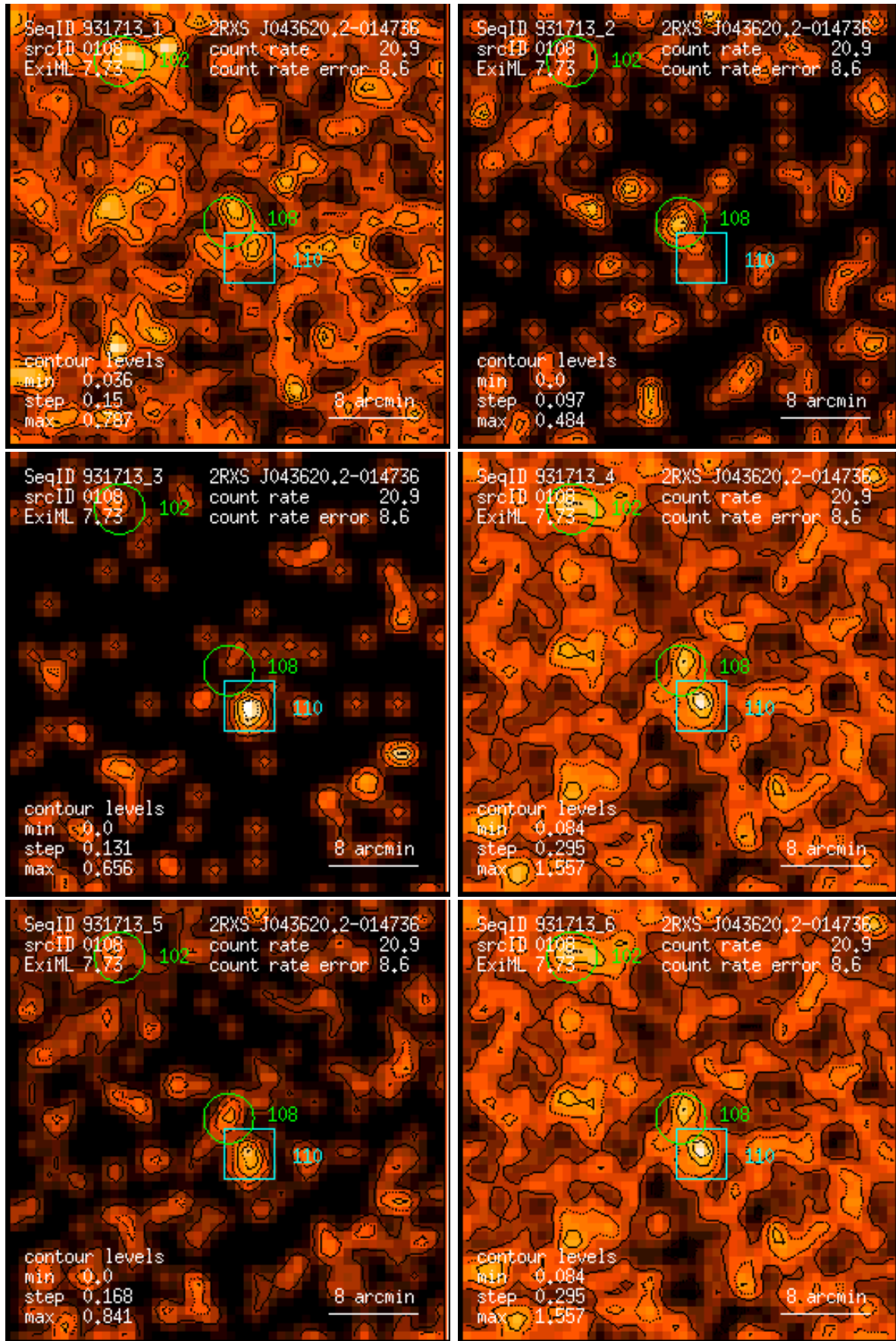
Figure 108: RASS 931713: detection 0108: band rate images, Gaussian filter: (1) PSPC channels 11 – 41, (2) 52 – 90, (3) 91 – 201, (4) 11 – 235, (5) 52 – 201, (6) 11 – 201. Broad band rates in counts/ks. Band rate contour levels in counts/ks/arcmin 2 .
