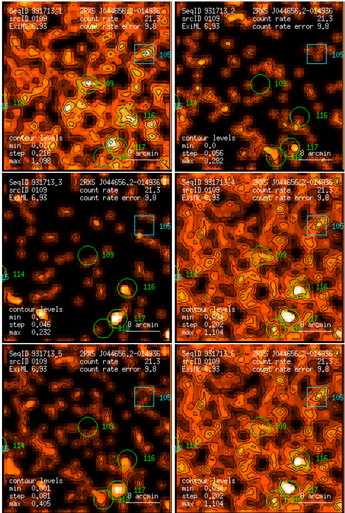
Figure 109: RASS 931713: detection 0109: band rate images, Gaussian filter: (1) PSPC channels 11 – 41, (2) 52 – 90, (3) 91 – 201, (4) 11 – 235, (5) 52 – 201, (6) 11 – 201. Broad band rates in counts/ks. Band rate contour levels in counts/ks/arcmin 2 .
