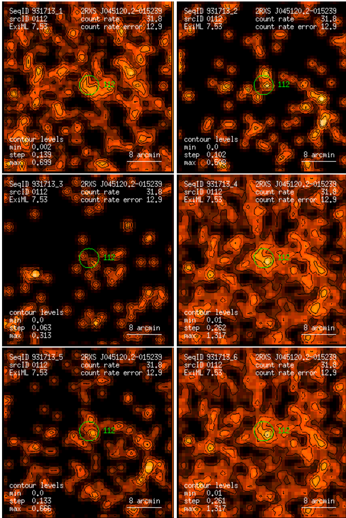
Figure 112: RASS 931713: detection 0112: band rate images, Gaussian filter: (1) PSPC channels 11 – 41, (2) 52 – 90, (3) 91 – 201, (4) 11 – 235, (5) 52 – 201, (6) 11 – 201. Broad band rates in counts/ks. Band rate contour levels in counts/ks/arcmin 2 .
