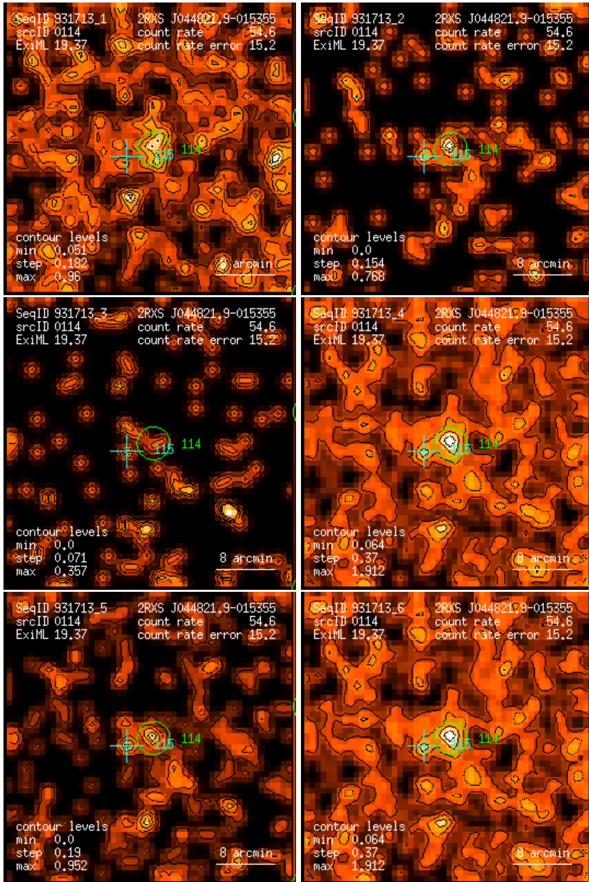
Figure 114: RASS 931713: detection 0114: band rate images, Gaussian filter: (1) PSPC channels 11 – 41, (2) 52 – 90, (3) 91 – 201, (4) 11 – 235, (5) 52 – 201, (6) 11 – 201. Broad band rates in counts/ks. Band rate contour levels in counts/ks/arcmin 2 .
