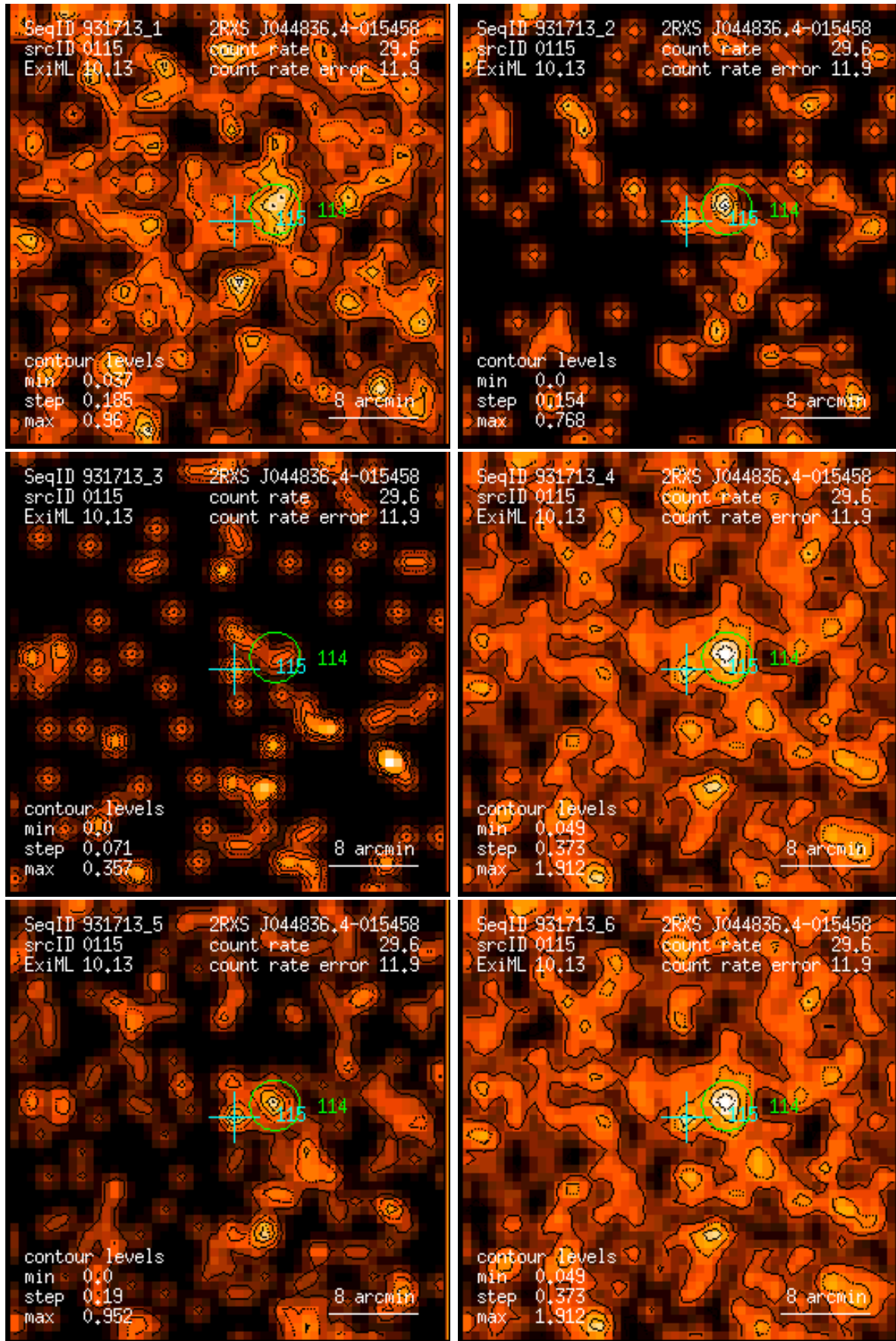
Figure 115: RASS 931713: detection 0115: band rate images, Gaussian filter: (1) PSPC channels 11 – 41, (2) 52 – 90, (3) 91 – 201, (4) 11 – 235, (5) 52 – 201, (6) 11 – 201. Broad band rates in counts/ks. Band rate contour levels in counts/ks/arcmin 2 .
