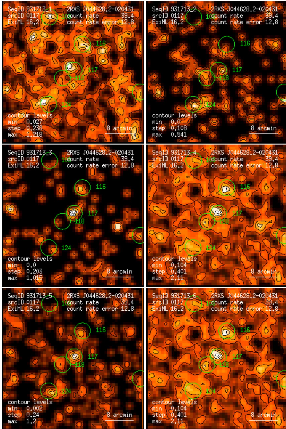
Figure 117: RASS 931713: detection 0117: band rate images, Gaussian filter: (1) PSPC channels 11 – 41, (2) 52 – 90, (3) 91 – 201, (4) 11 – 235, (5) 52 – 201, (6) 11 – 201. Broad band rates in counts/ks. Band rate contour levels in counts/ks/arcmin 2 .
