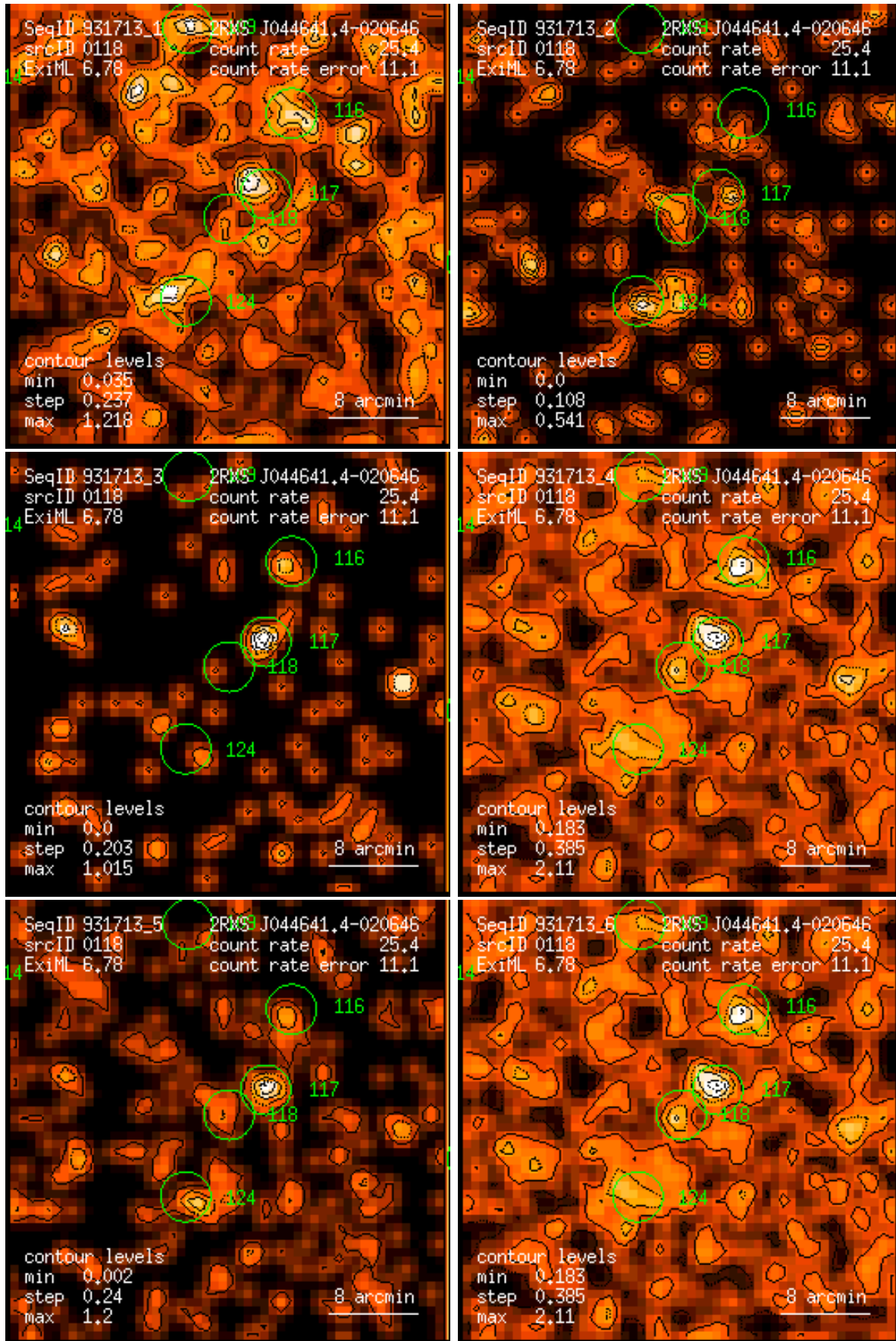
Figure 118: RASS 931713: detection 0118: band rate images, Gaussian filter: (1) PSPC channels 11 – 41, (2) 52 – 90, (3) 91 – 201, (4) 11 – 235, (5) 52 – 201, (6) 11 – 201. Broad band rates in counts/ks. Band rate contour levels in counts/ks/arcmin 2 .
