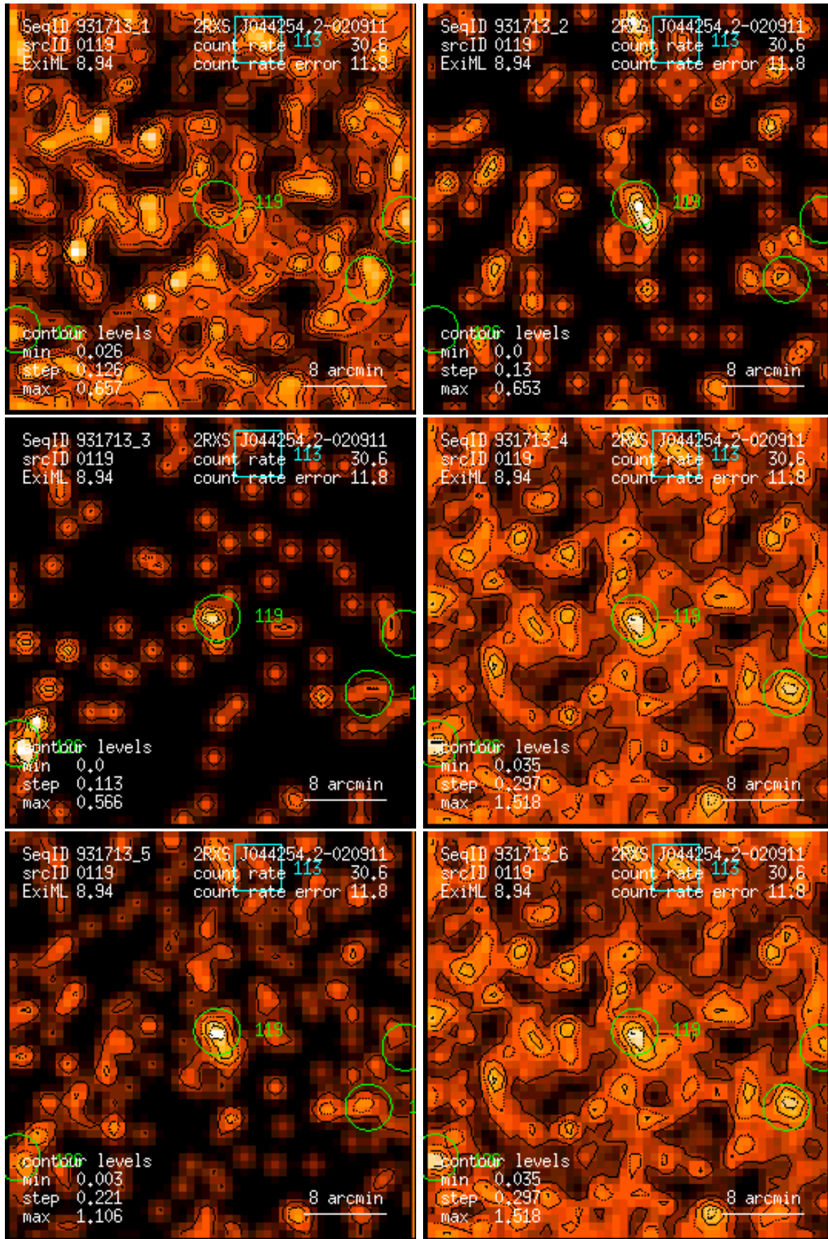
Figure 119: RASS 931713: detection 0119: band rate images, Gaussian filter: (1) PSPC channels 11 – 41, (2) 52 – 90, (3) 91 – 201, (4) 11 – 235, (5) 52 – 201, (6) 11 – 201. Broad band rates in counts/ks. Band rate contour levels in counts/ks/arcmin 2 .
