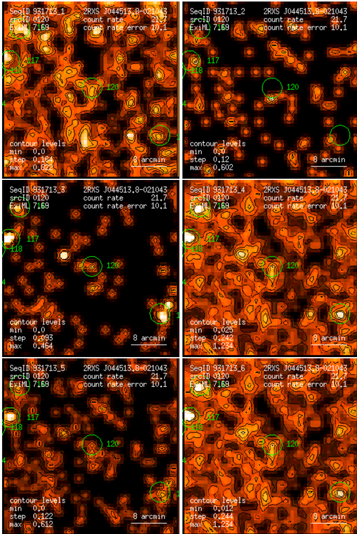
Figure 120: RASS 931713: detection 0120: band rate images, Gaussian filter: (1) PSPC channels 11 – 41, (2) 52 – 90, (3) 91 – 201, (4) 11 – 235, (5) 52 – 201, (6) 11 – 201. Broad band rates in counts/ks. Band rate contour levels in counts/ks/arcmin 2 .
