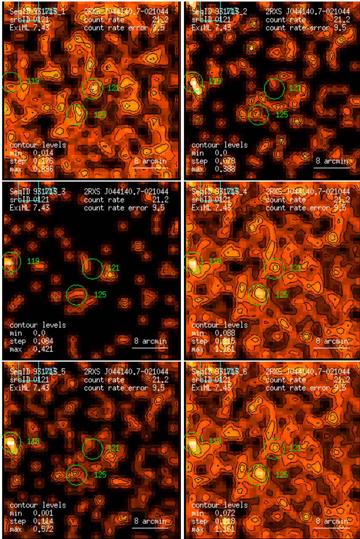
Figure 121: RASS 931713: detection 0121: band rate images, Gaussian filter: (1) PSPC channels 11 – 41, (2) 52 – 90, (3) 91 – 201, (4) 11 – 235, (5) 52 – 201, (6) 11 – 201. Broad band rates in counts/ks. Band rate contour levels in counts/ks/arcmin 2 .
