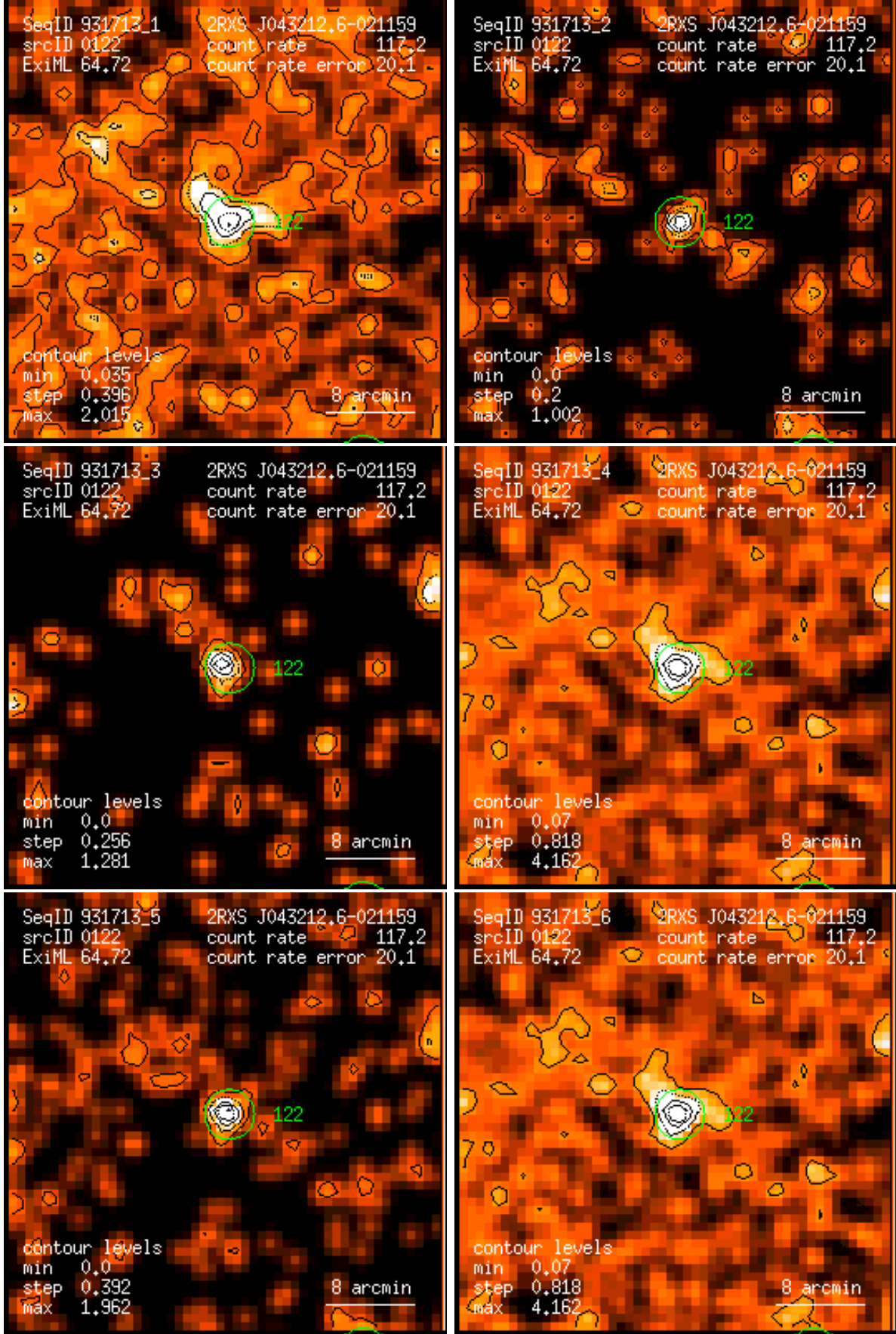
Figure 122: RASS 931713: detection 0122: band rate images, Gaussian filter: (1) PSPC channels 11 – 41, (2) 52 – 90, (3) 91 – 201, (4) 11 – 235, (5) 52 – 201, (6) 11 – 201. Broad band rates in counts/ks. Band rate contour levels in counts/ks/arcmin 2 .
