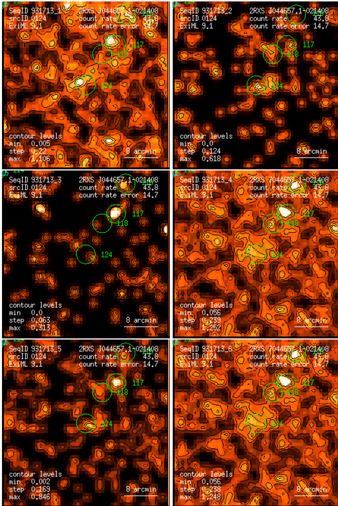
Figure 124: RASS 931713: detection 0124: band rate images, Gaussian filter: (1) PSPC channels 11 – 41, (2) 52 – 90, (3) 91 – 201, (4) 11 – 235, (5) 52 – 201, (6) 11 – 201. Broad band rates in counts/ks. Band rate contour levels in counts/ks/arcmin 2 .
