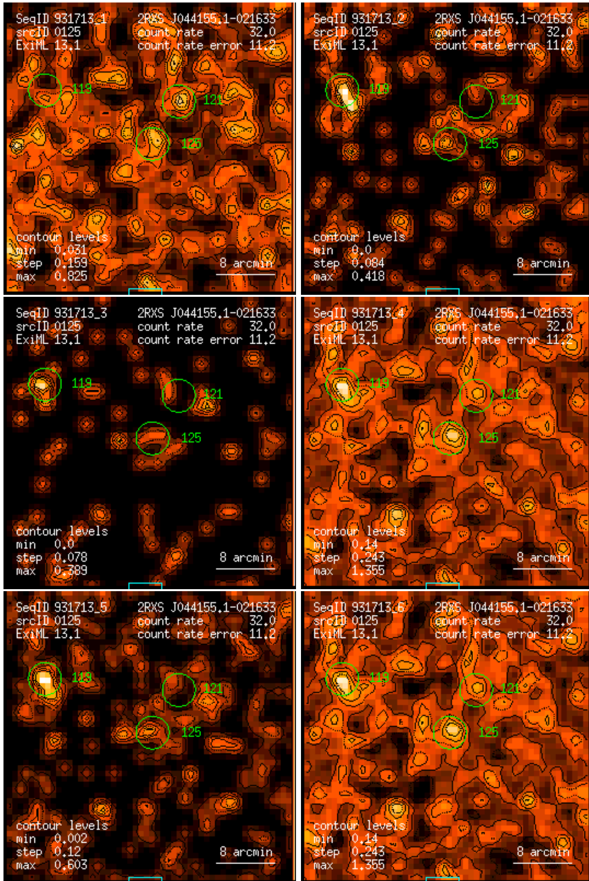
Figure 125: RASS 931713: detection 0125: band rate images, Gaussian filter: (1) PSPC channels 11 – 41, (2) 52 – 90, (3) 91 – 201, (4) 11 – 235, (5) 52 – 201, (6) 11 – 201. Broad band rates in counts/ks. Band rate contour levels in counts/ks/arcmin 2 .
