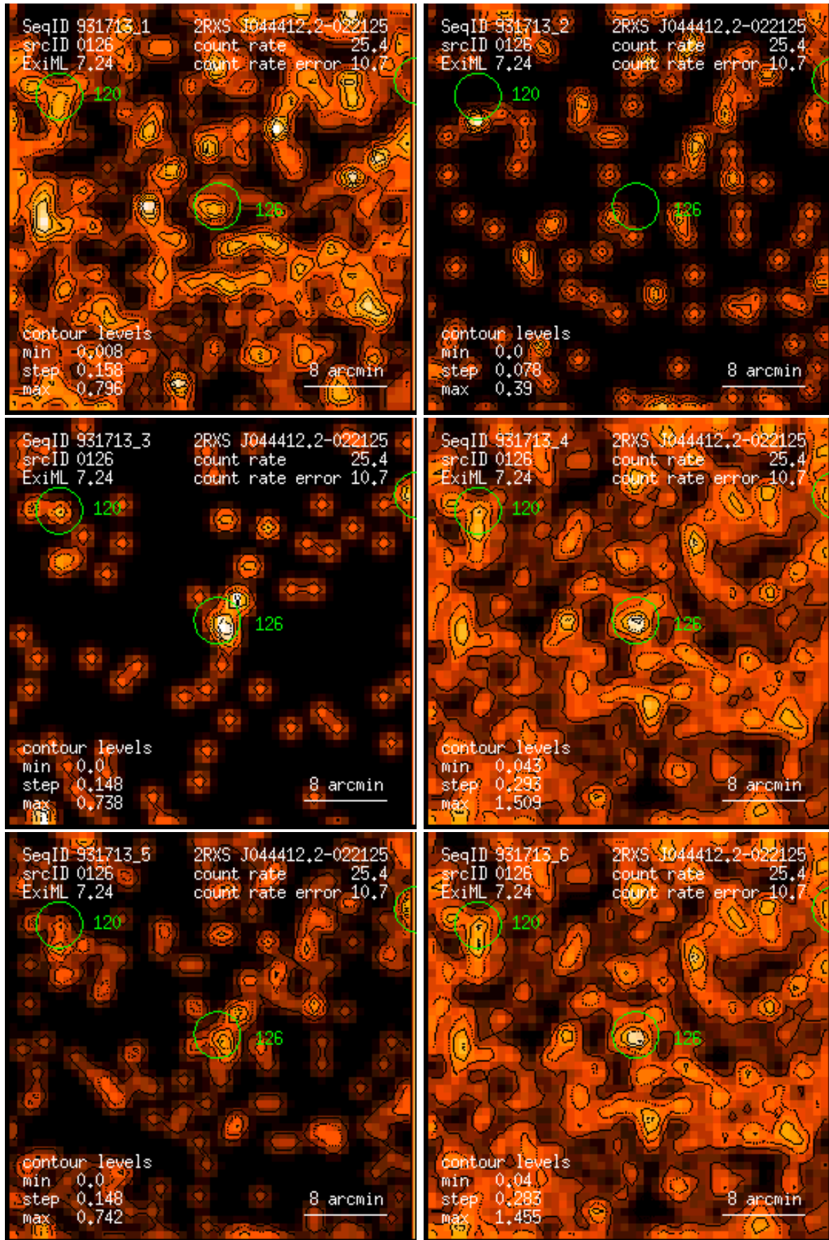
Figure 126: RASS 931713: detection 0126: band rate images, Gaussian filter: (1) PSPC channels 11 – 41, (2) 52 – 90, (3) 91 – 201, (4) 11 – 235, (5) 52 – 201, (6) 11 – 201. Broad band rates in counts/ks. Band rate contour levels in counts/ks/arcmin 2 .
