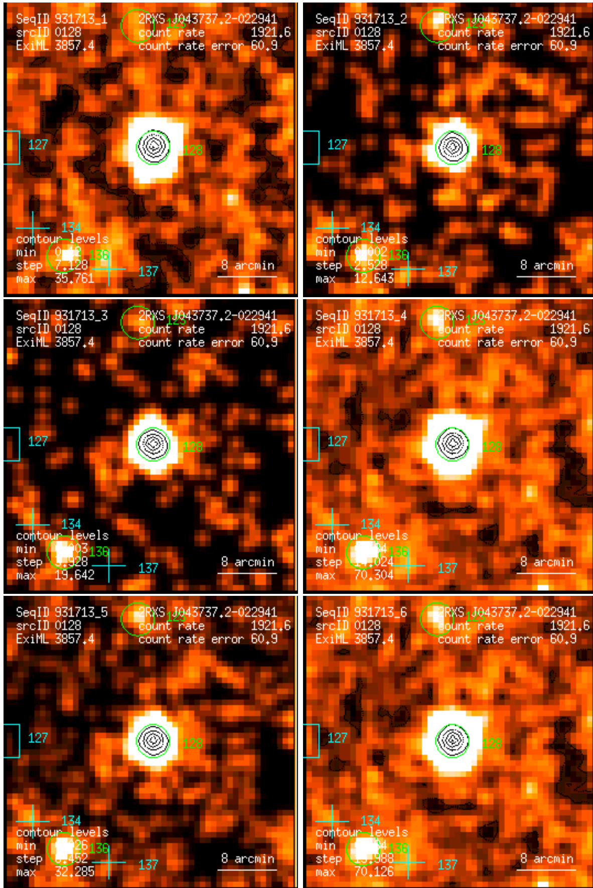
Figure 128: RASS 931713: detection 0128: band rate images, Gaussian filter: (1) PSPC channels 11 – 41, (2) 52 – 90, (3) 91 – 201, (4) 11 – 235, (5) 52 – 201, (6) 11 – 201. Broad band rates in counts/ks. Band rate contour levels in counts/ks/arcmin 2 .
