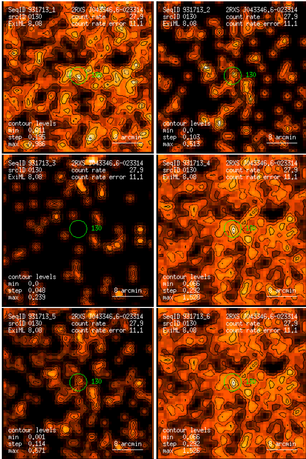
Figure 130: RASS 931713: detection 0130: band rate images, Gaussian filter: (1) PSPC channels 11 – 41, (2) 52 – 90, (3) 91 – 201, (4) 11 – 235, (5) 52 – 201, (6) 11 – 201. Broad band rates in counts/ks. Band rate contour levels in counts/ks/arcmin 2 .
