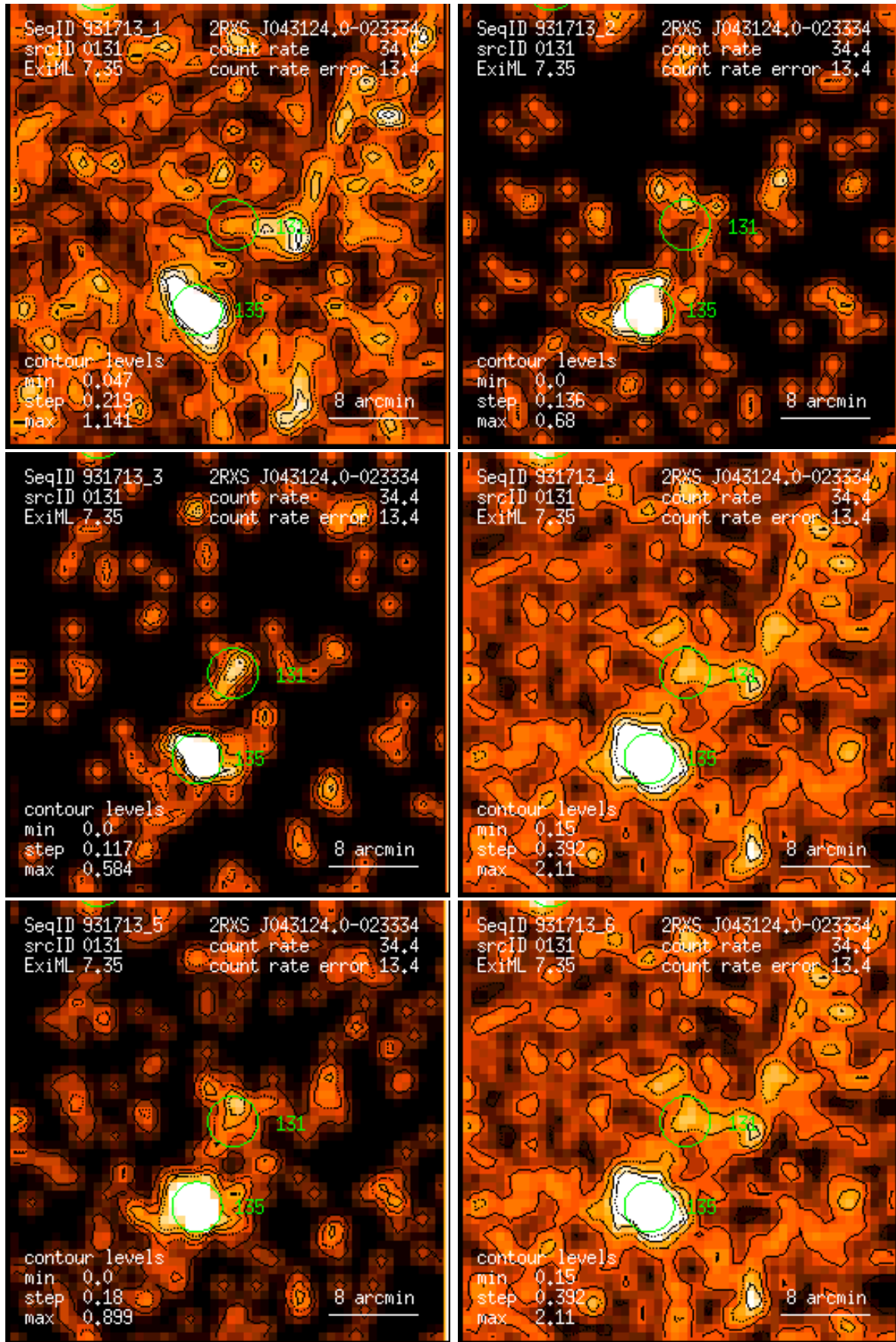
Figure 131: RASS 931713: detection 0131: band rate images, Gaussian filter: (1) PSPC channels 11 – 41, (2) 52 – 90, (3) 91 – 201, (4) 11 – 235, (5) 52 – 201, (6) 11 – 201. Broad band rates in counts/ks. Band rate contour levels in counts/ks/arcmin 2 .
