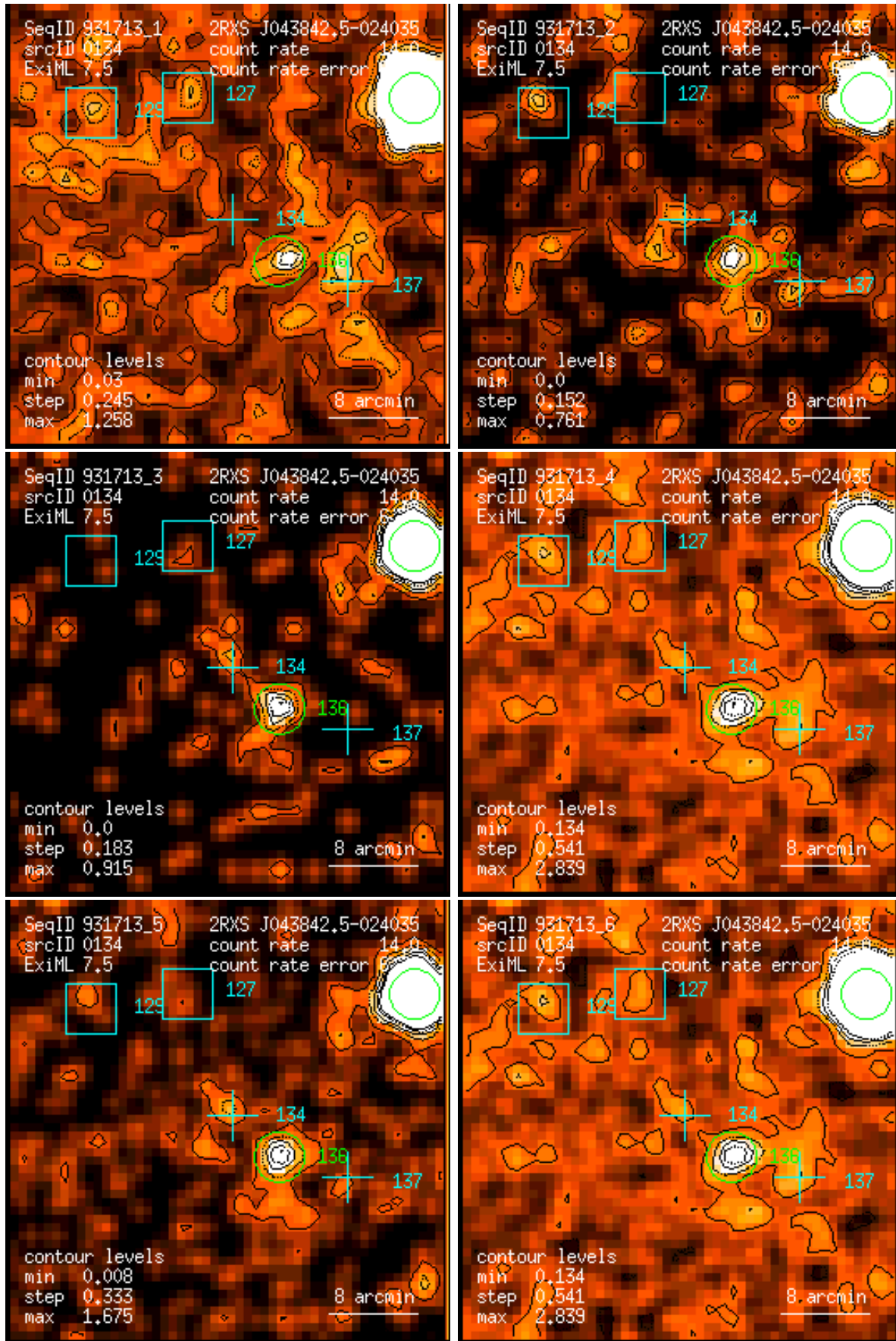
Figure 134: RASS 931713: detection 0134: band rate images, Gaussian filter: (1) PSPC channels 11 – 41, (2) 52 – 90, (3) 91 – 201, (4) 11 – 235, (5) 52 – 201, (6) 11 – 201. Broad band rates in counts/ks. Band rate contour levels in counts/ks/arcmin 2 .
