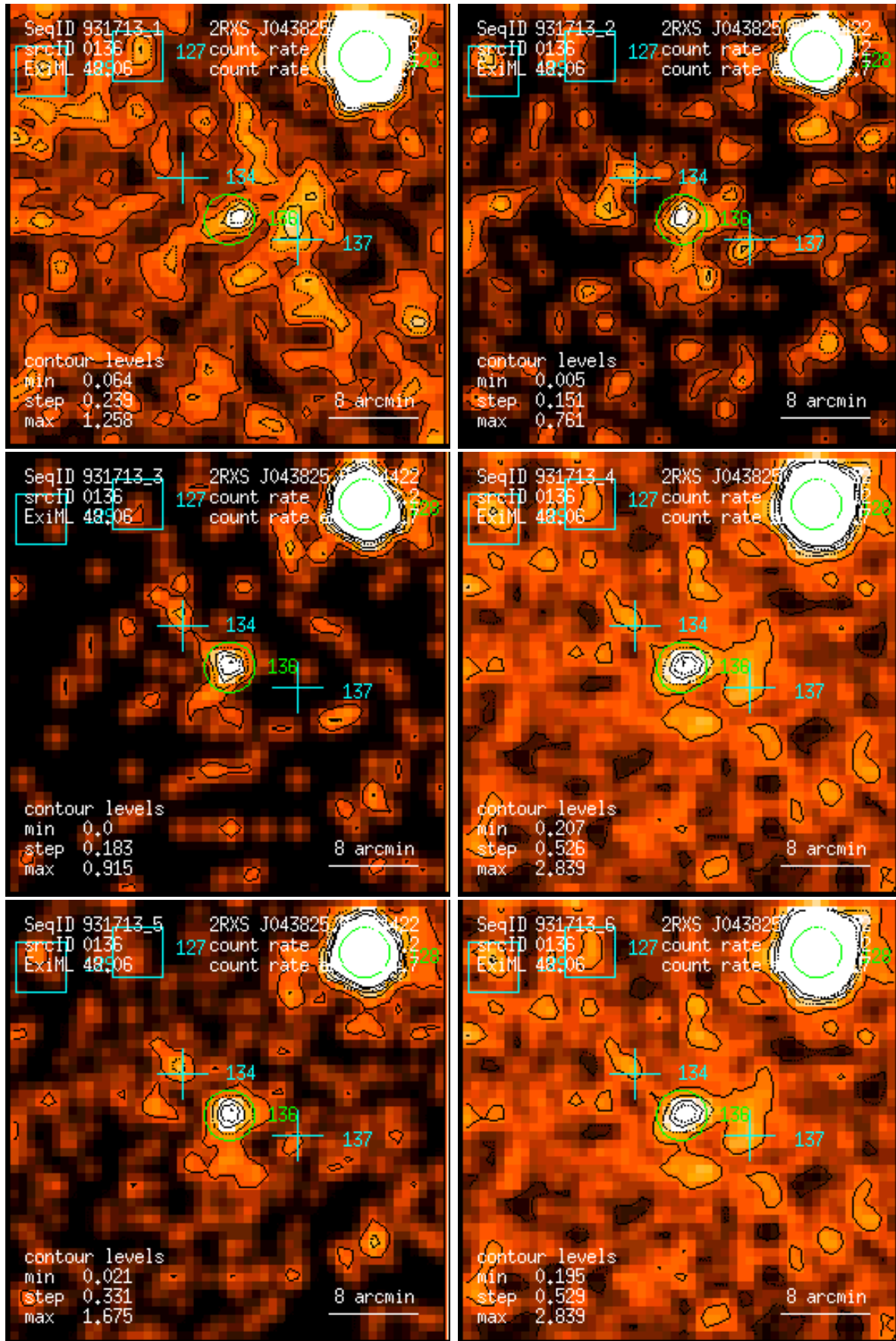
Figure 136: RASS 931713: detection 0136: band rate images, Gaussian filter: (1) PSPC channels 11 – 41, (2) 52 – 90, (3) 91 – 201, (4) 11 – 235, (5) 52 – 201, (6) 11 – 201. Broad band rates in counts/ks. Band rate contour levels in counts/ks/arcmin 2 .
