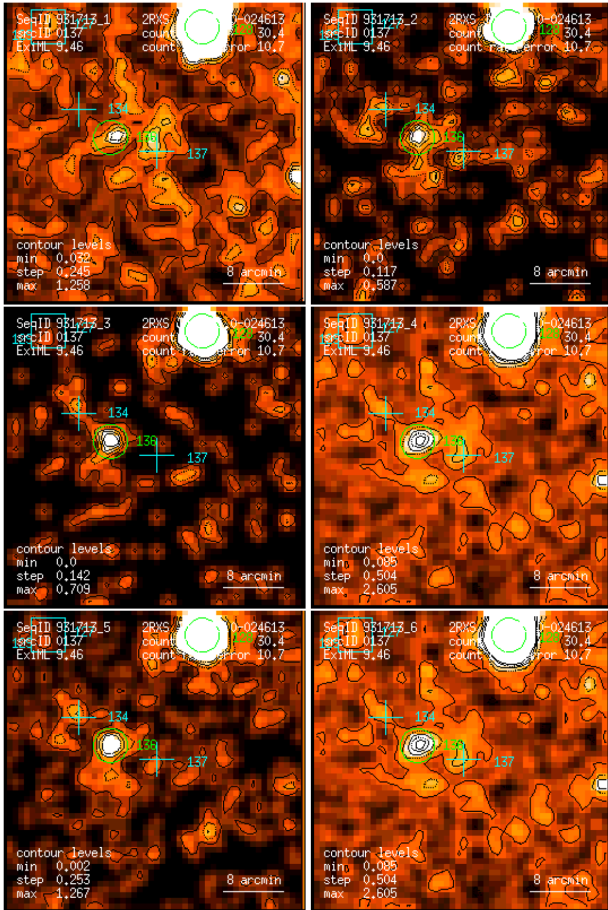
Figure 137: RASS 931713: detection 0137: band rate images, Gaussian filter: (1) PSPC channels 11 – 41, (2) 52 – 90, (3) 91 – 201, (4) 11 – 235, (5) 52 – 201, (6) 11 – 201. Broad band rates in counts/ks. Band rate contour levels in counts/ks/arcmin 2 .
