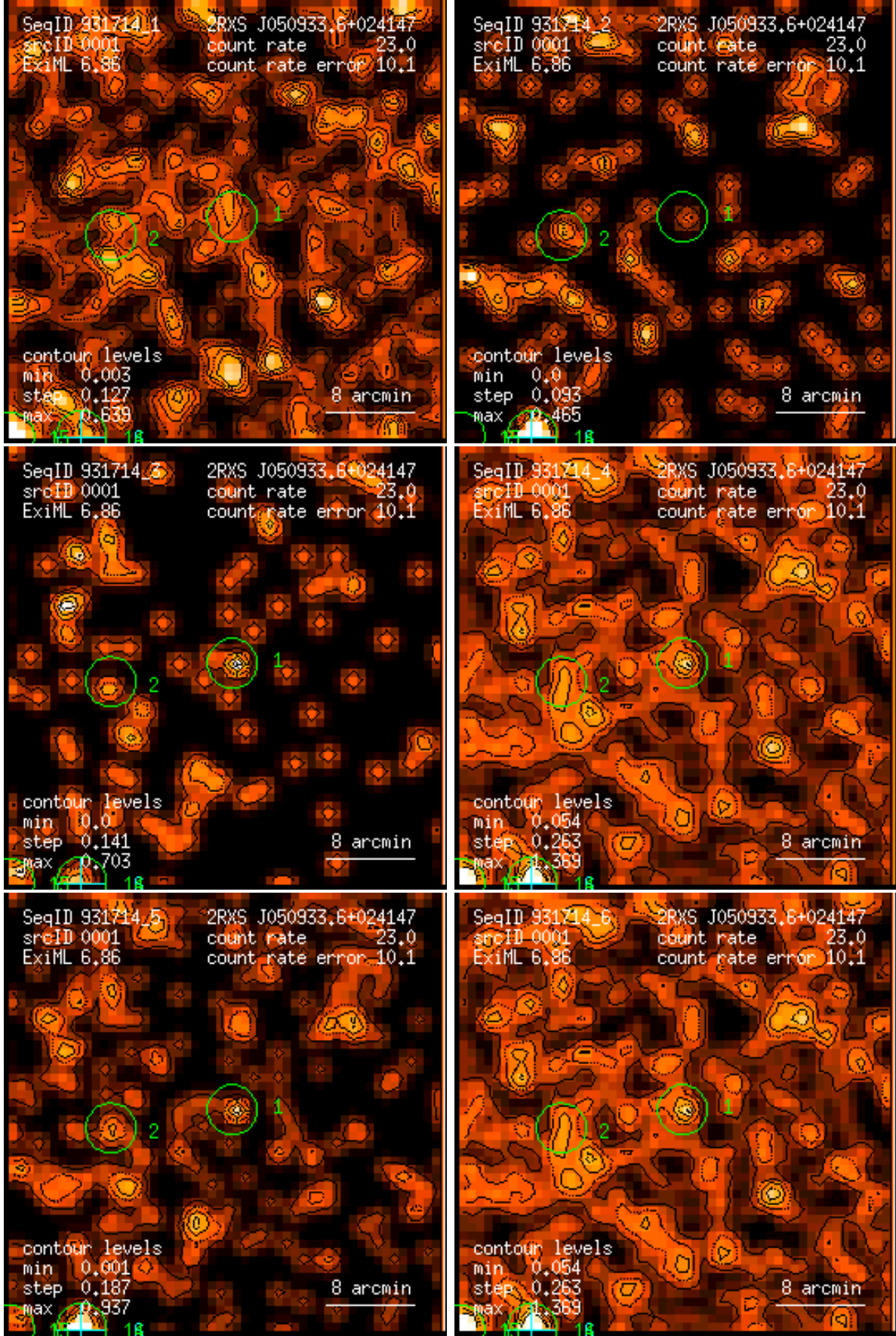
Figure 1: RASS 931714: detection 0001: band rate images, Gaussian filter: (1) PSPC channels 11 – 41, (2) 52 – 90, (3) 91 – 201, (4) 11 – 235, (5) 52 – 201, (6) 11 – 201. Broad band rates in counts/ks. Band rate contour levels in counts/ks/arcmin 2 .
