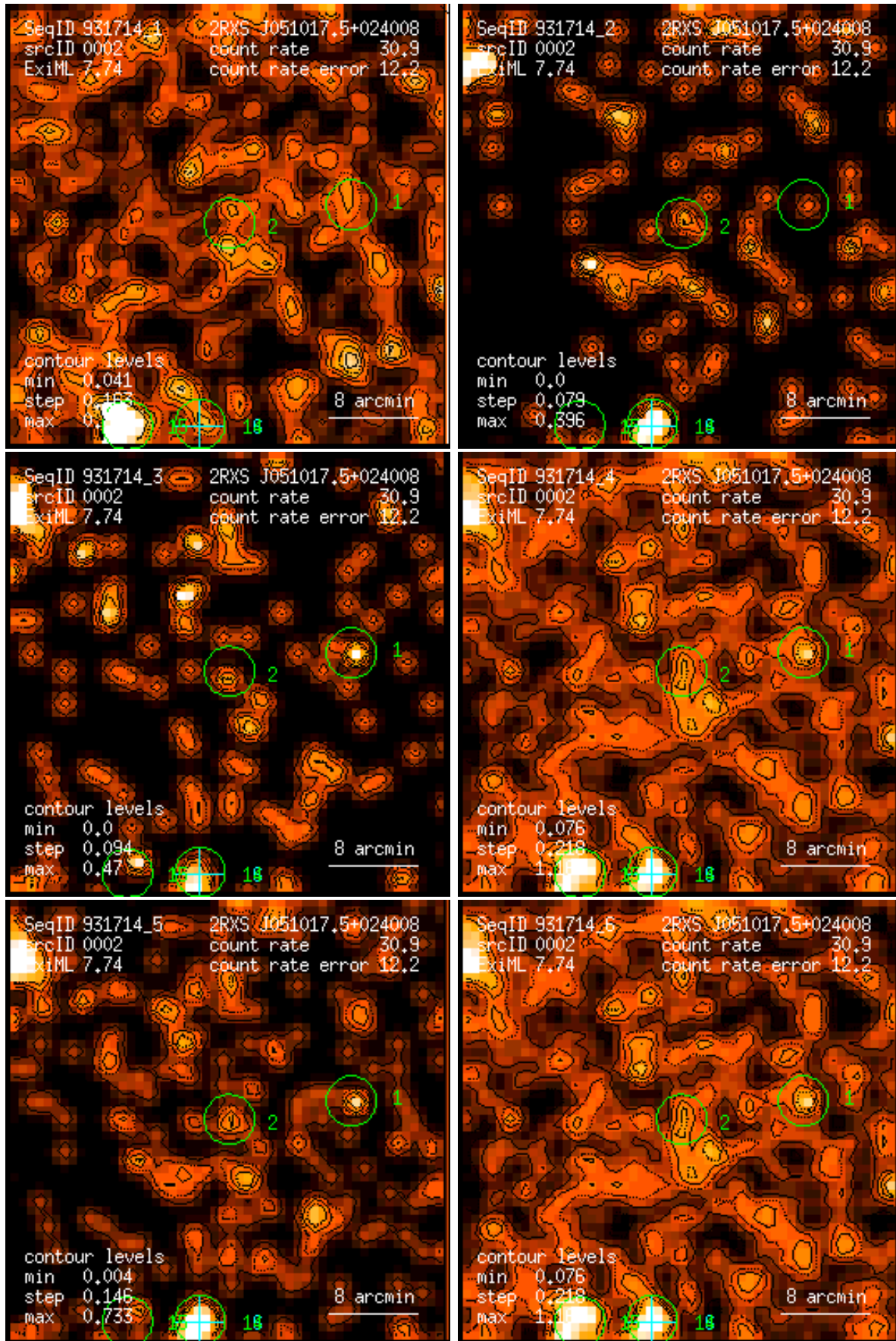
Figure 2: RASS 931714: detection 0002: band rate images, Gaussian filter: (1) PSPC channels 11 – 41, (2) 52 – 90, (3) 91 – 201, (4) 11 – 235, (5) 52 – 201, (6) 11 – 201. Broad band rates in counts/ks. Band rate contour levels in counts/ks/arcmin 2 .
