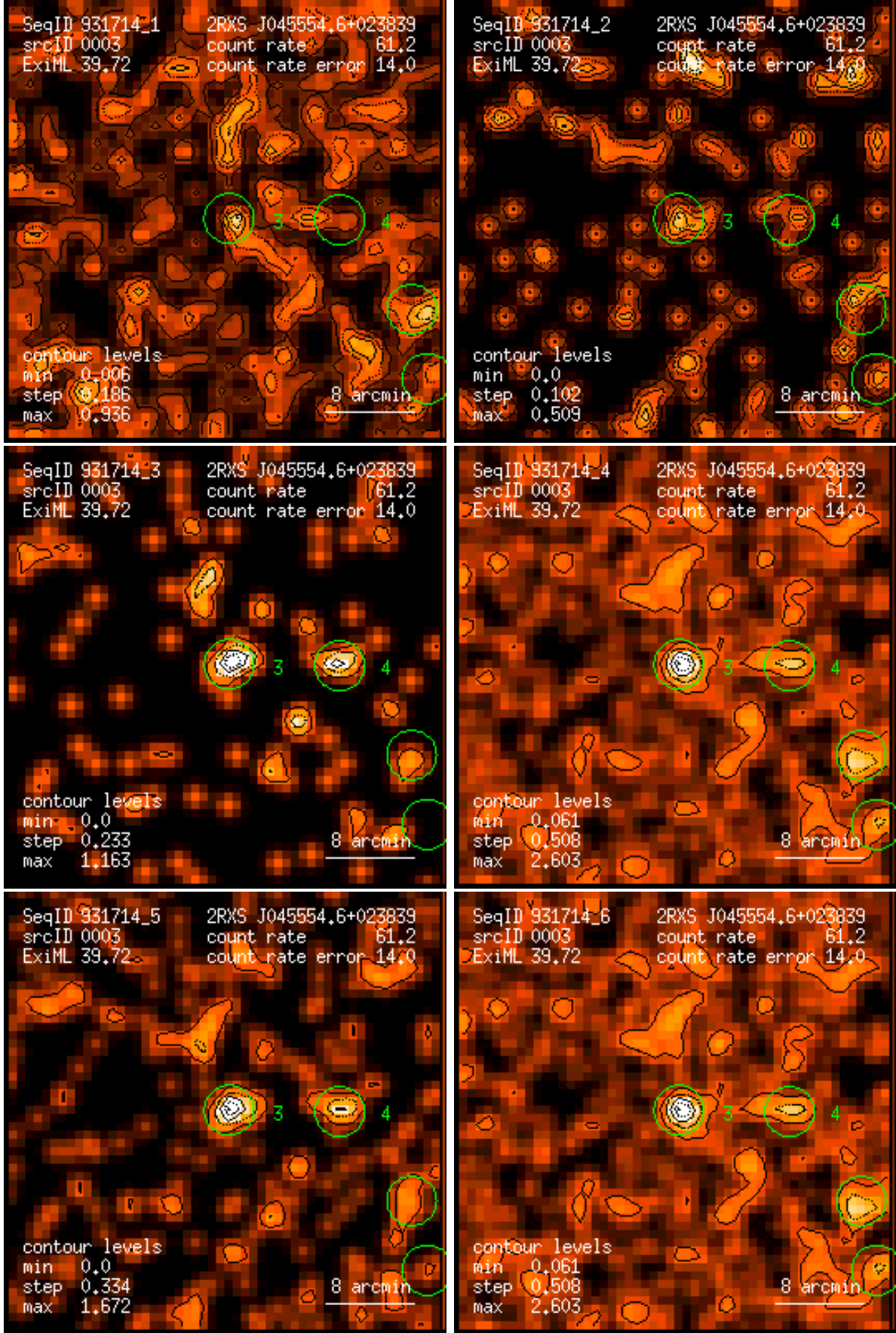
Figure 3: RASS 931714: detection 0003: band rate images, Gaussian filter: (1) PSPC channels 11 – 41, (2) 52 – 90, (3) 91 – 201, (4) 11 – 235, (5) 52 – 201, (6) 11 – 201. Broad band rates in counts/ks. Band rate contour levels in counts/ks/arcmin 2 .
