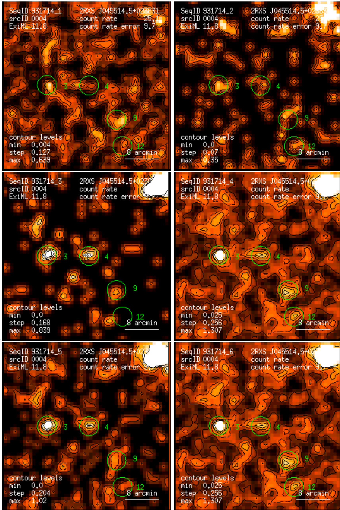
Figure 4: RASS 931714: detection 0004: band rate images, Gaussian filter: (1) PSPC channels 11 – 41, (2) 52 – 90, (3) 91 – 201, (4) 11 – 235, (5) 52 – 201, (6) 11 – 201. Broad band rates in counts/ks. Band rate contour levels in counts/ks/arcmin 2 .
