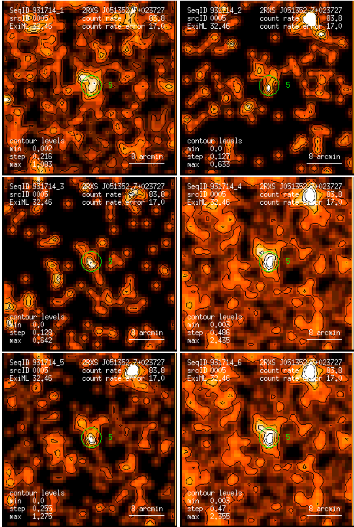
Figure 5: RASS 931714: detection 0005: band rate images, Gaussian filter: (1) PSPC channels 11 – 41, (2) 52 – 90, (3) 91 – 201, (4) 11 – 235, (5) 52 – 201, (6) 11 – 201. Broad band rates in counts/ks. Band rate contour levels in counts/ks/arcmin 2 .
