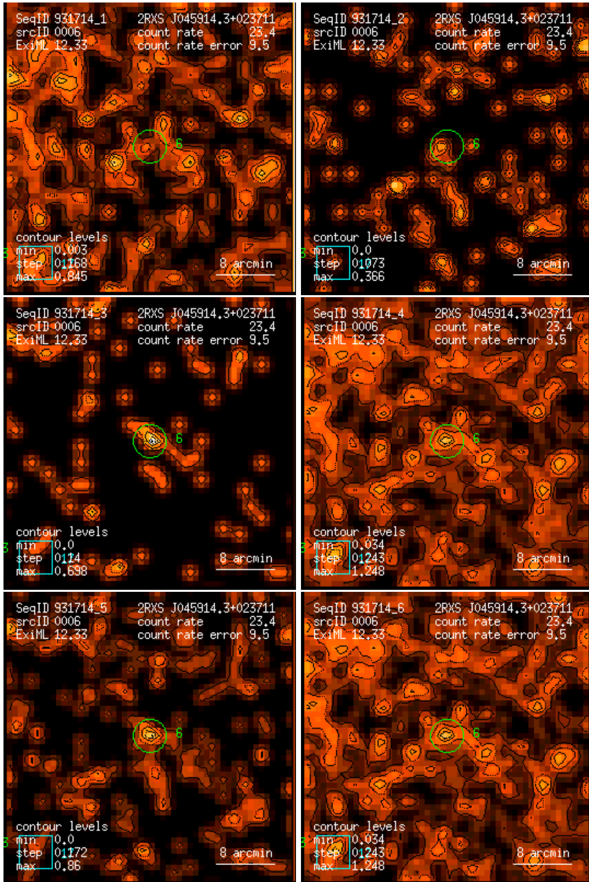
Figure 6: RASS 931714: detection 0006: band rate images, Gaussian filter: (1) PSPC channels 11 – 41, (2) 52 – 90, (3) 91 – 201, (4) 11 – 235, (5) 52 – 201, (6) 11 – 201. Broad band rates in counts/ks. Band rate contour levels in counts/ks/arcmin 2 .
