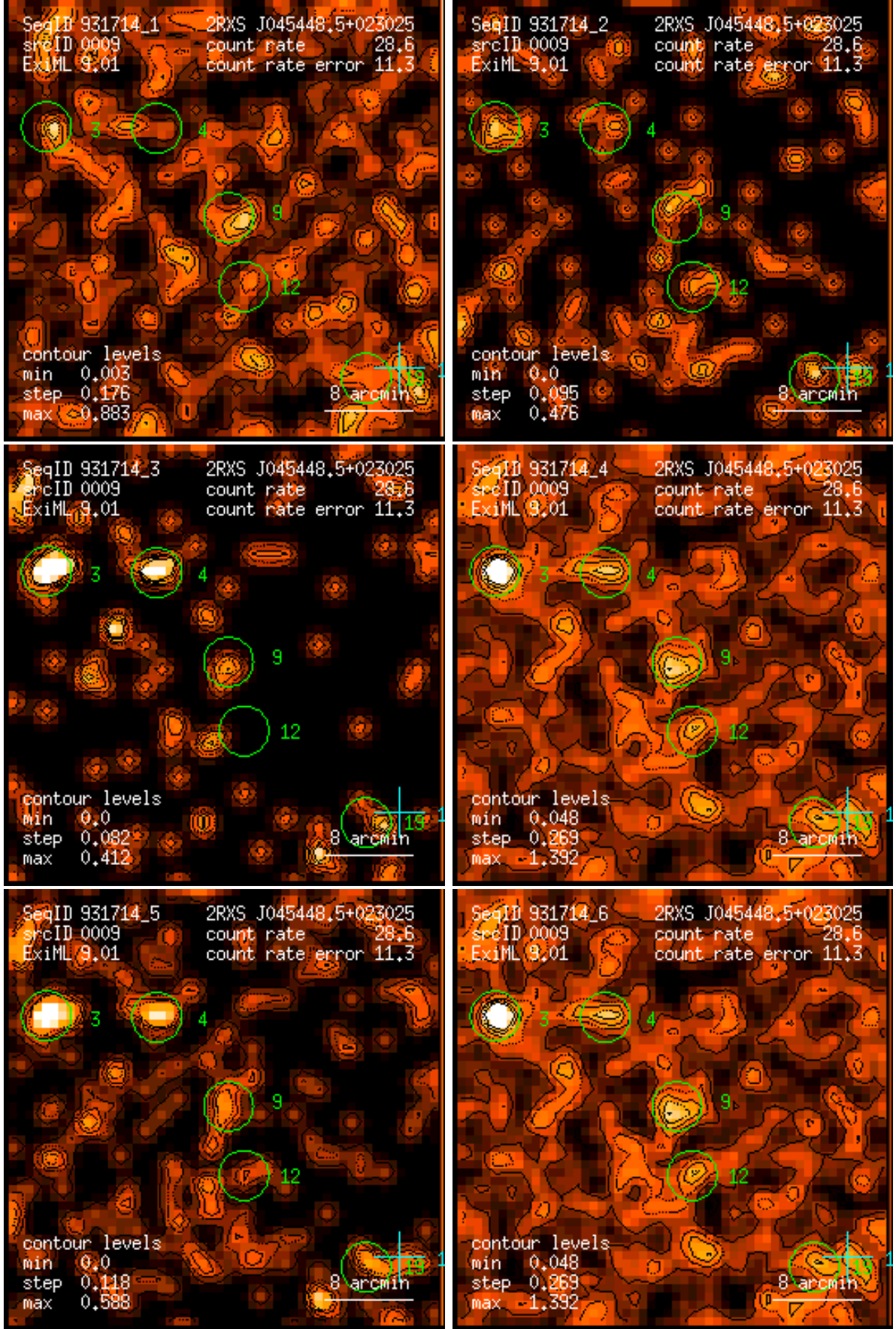
Figure 9: RASS 931714: detection 0009: band rate images, Gaussian filter: (1) PSPC channels 11 – 41, (2) 52 – 90, (3) 91 – 201, (4) 11 – 235, (5) 52 – 201, (6) 11 – 201. Broad band rates in counts/ks. Band rate contour levels in counts/ks/arcmin 2 .
