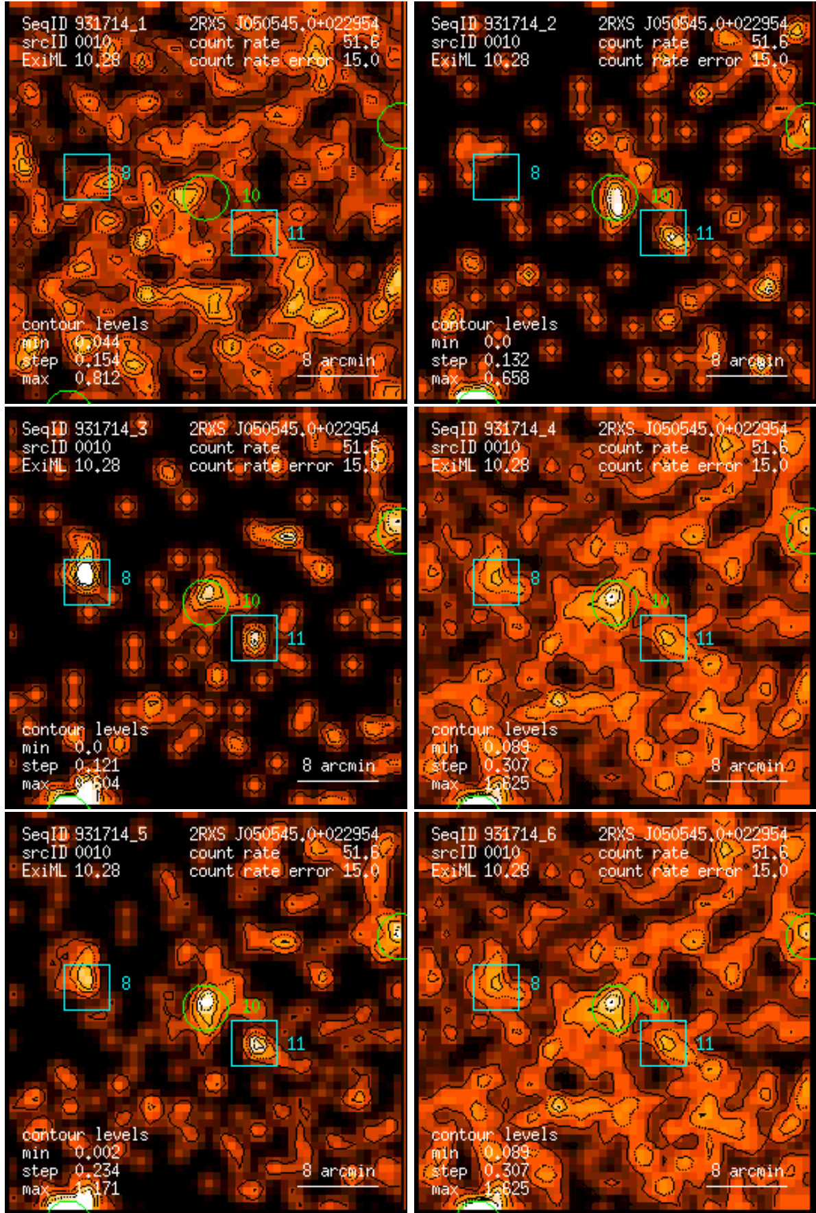
Figure 10: RASS 931714: detection 0010: band rate images, Gaussian filter: (1) PSPC channels 11 – 41, (2) 52 – 90, (3) 91 – 201, (4) 11 – 235, (5) 52 – 201, (6) 11 – 201. Broad band rates in counts/ks. Band rate contour levels in counts/ks/arcmin 2 .
