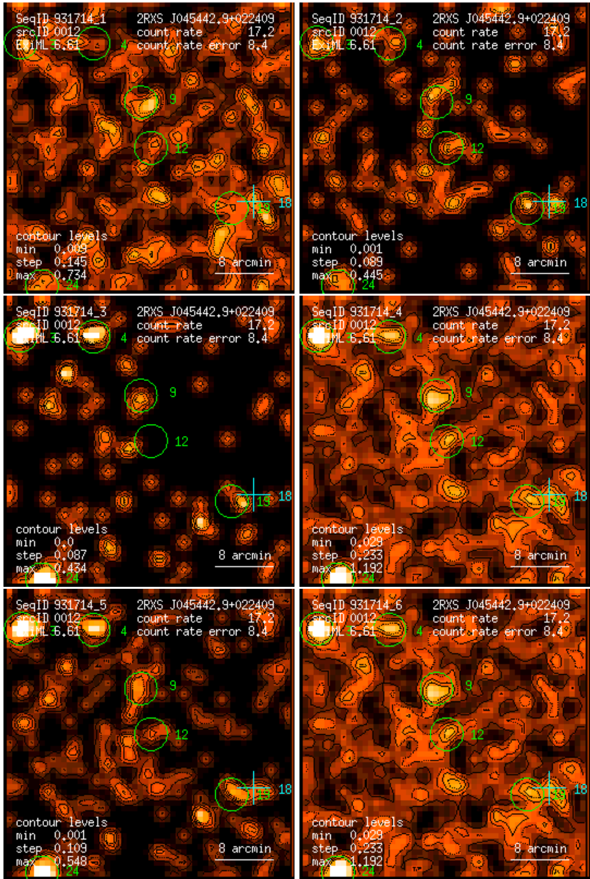
Figure 12: RASS 931714: detection 0012: band rate images, Gaussian filter: (1) PSPC channels 11 – 41, (2) 52 – 90, (3) 91 – 201, (4) 11 – 235, (5) 52 – 201, (6) 11 – 201. Broad band rates in counts/ks. Band rate contour levels in counts/ks/arcmin 2 .
