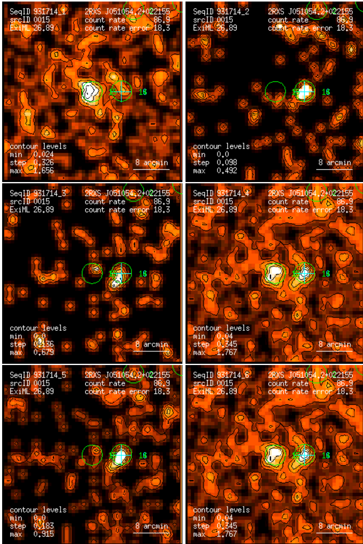
Figure 15: RASS 931714: detection 0015: band rate images, Gaussian filter: (1) PSPC channels 11 – 41, (2) 52 – 90, (3) 91 – 201, (4) 11 – 235, (5) 52 – 201, (6) 11 – 201. Broad band rates in counts/ks. Band rate contour levels in counts/ks/arcmin 2 .
