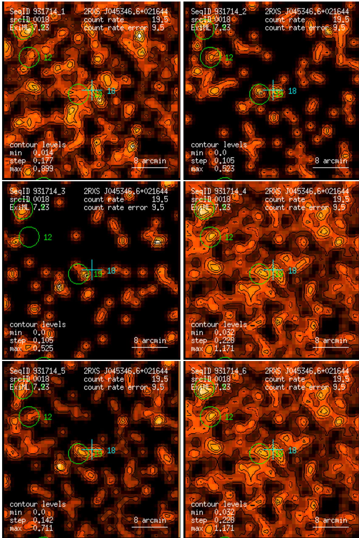
Figure 18: RASS 931714: detection 0018: band rate images, Gaussian filter: (1) PSPC channels 11 – 41, (2) 52 – 90, (3) 91 – 201, (4) 11 – 235, (5) 52 – 201, (6) 11 – 201. Broad band rates in counts/ks. Band rate contour levels in counts/ks/arcmin 2 .
